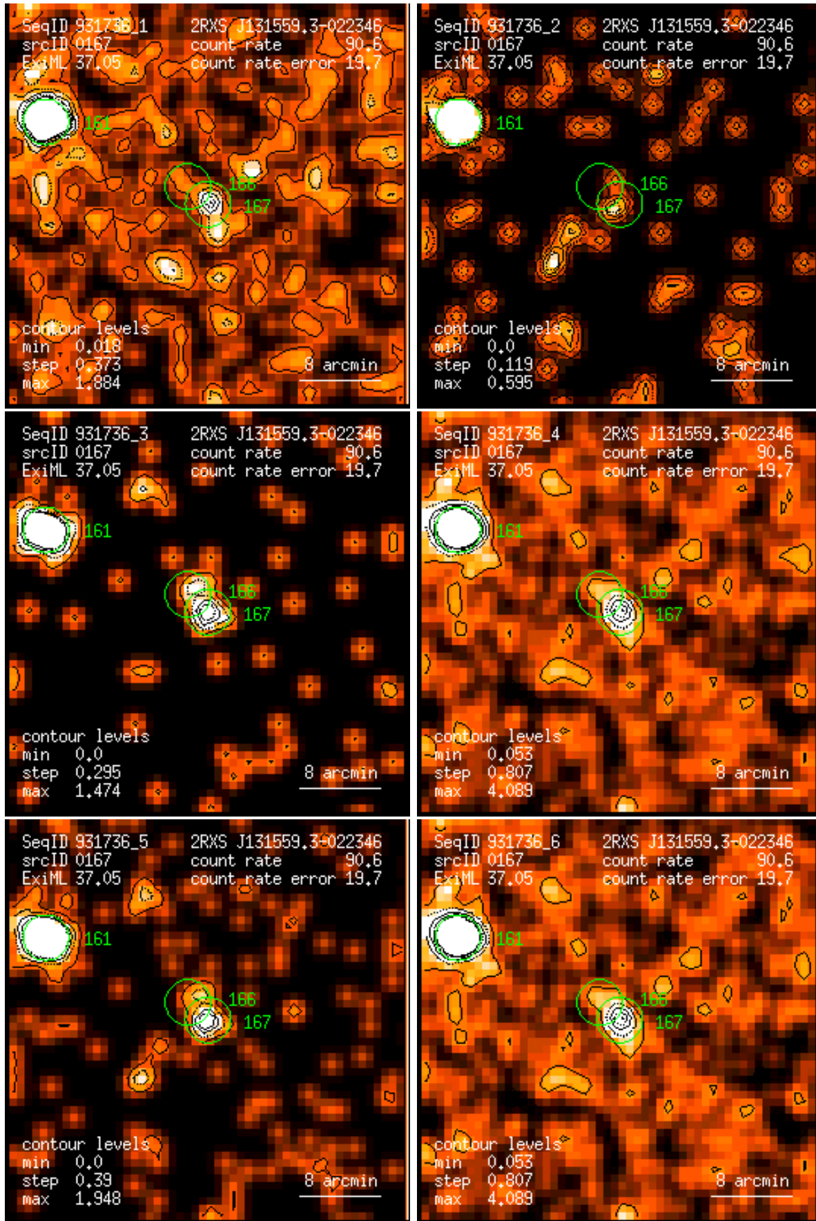
Figure 167: RASS 931736: detection 0167: band rate images, Gaussian filter: (1) PSPC channels 11 – 41, (2) 52 – 90, (3) 91 – 201, (4) 11 – 235, (5) 52 – 201, (6) 11 – 201. Broad band rates in counts/ks. Band rate contour levels in counts/ks/arcmin 2 .
