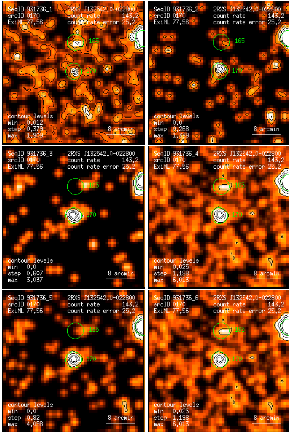
Figure 170: RASS 931736: detection 0170: band rate images, Gaussian filter: (1) PSPC channels 11 – 41, (2) 52 – 90, (3) 91 – 201, (4) 11 – 235, (5) 52 – 201, (6) 11 – 201. Broad band rates in counts/ks. Band rate contour levels in counts/ks/arcmin 2 .
