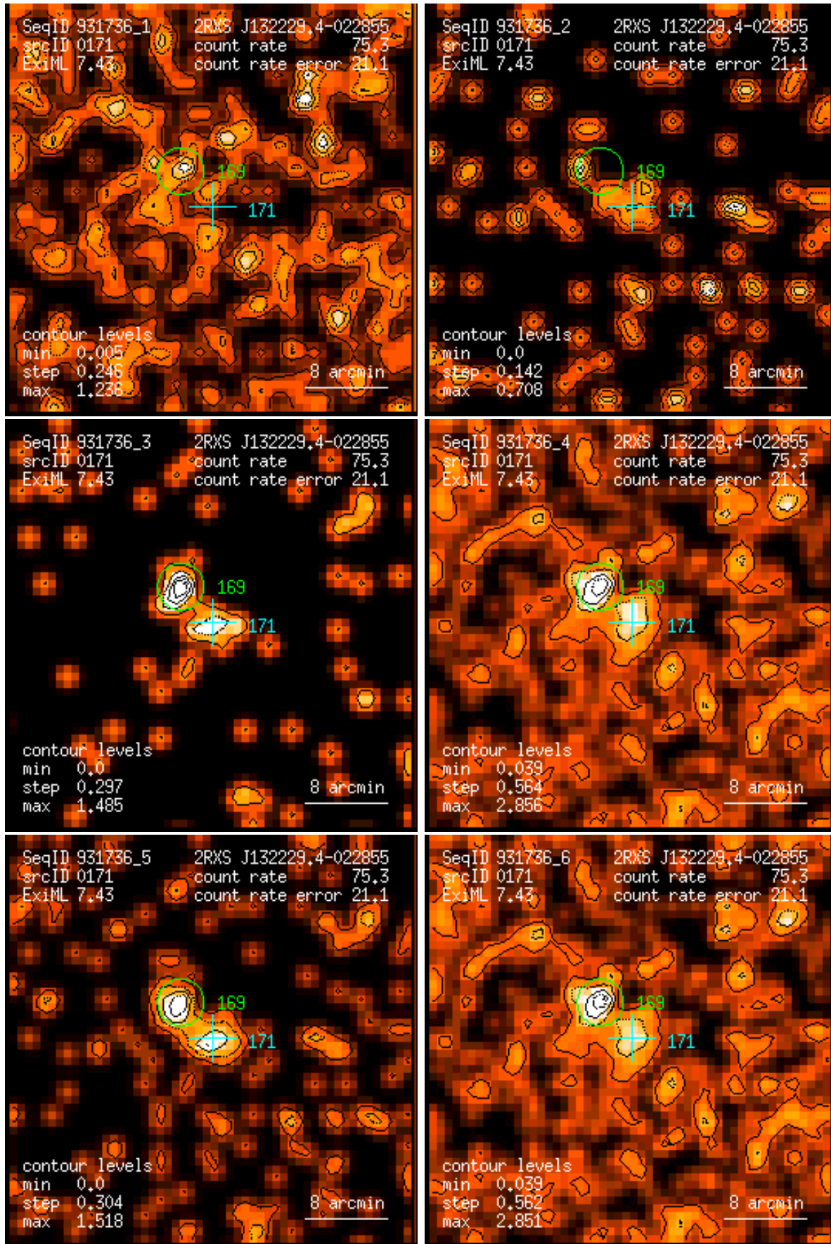
Figure 171: RASS 931736: detection 0171: band rate images, Gaussian filter: (1) PSPC channels 11 – 41, (2) 52 – 90, (3) 91 – 201, (4) 11 – 235, (5) 52 – 201, (6) 11 – 201. Broad band rates in counts/ks. Band rate contour levels in counts/ks/arcmin 2 .
