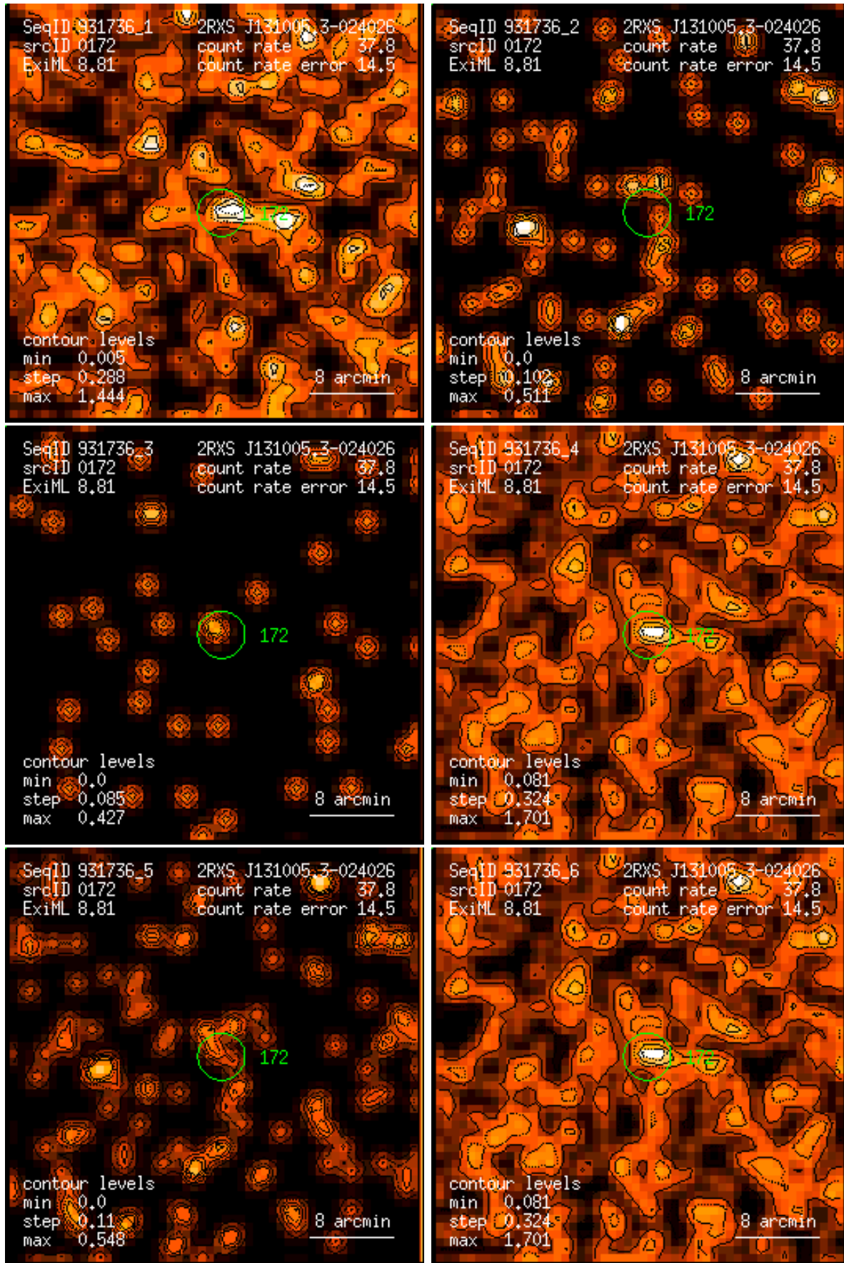
Figure 172: RASS 931736: detection 0172: band rate images, Gaussian filter: (1) PSPC channels 11 – 41, (2) 52 – 90, (3) 91 – 201, (4) 11 – 235, (5) 52 – 201, (6) 11 – 201. Broad band rates in counts/ks. Band rate contour levels in counts/ks/arcmin 2 .
