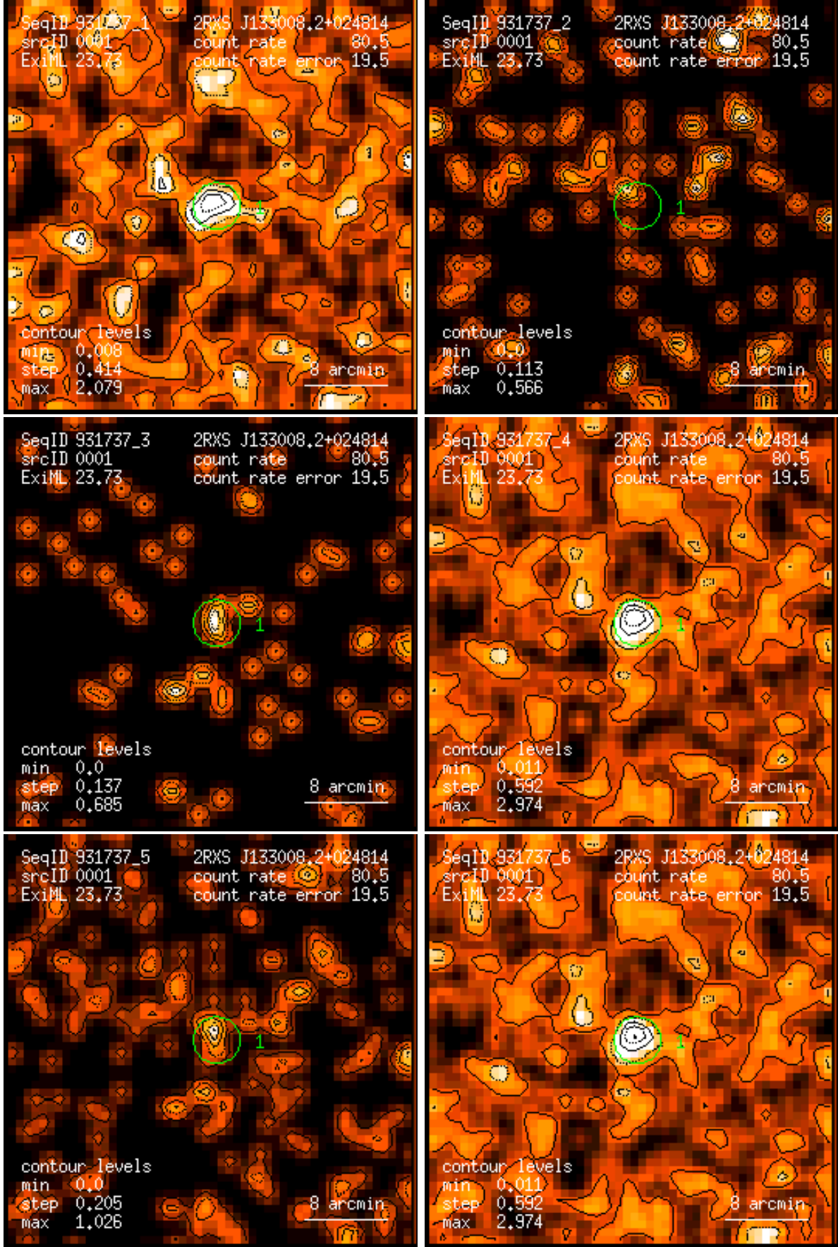
Figure 1: RASS 931737: detection 0001: band rate images, Gaussian filter: (1) PSPC channels 11 – 41, (2) 52 – 90, (3) 91 – 201, (4) 11 – 235, (5) 52 – 201, (6) 11 – 201. Broad band rates in counts/ks. Band rate contour levels in counts/ks/arcmin 2 .
