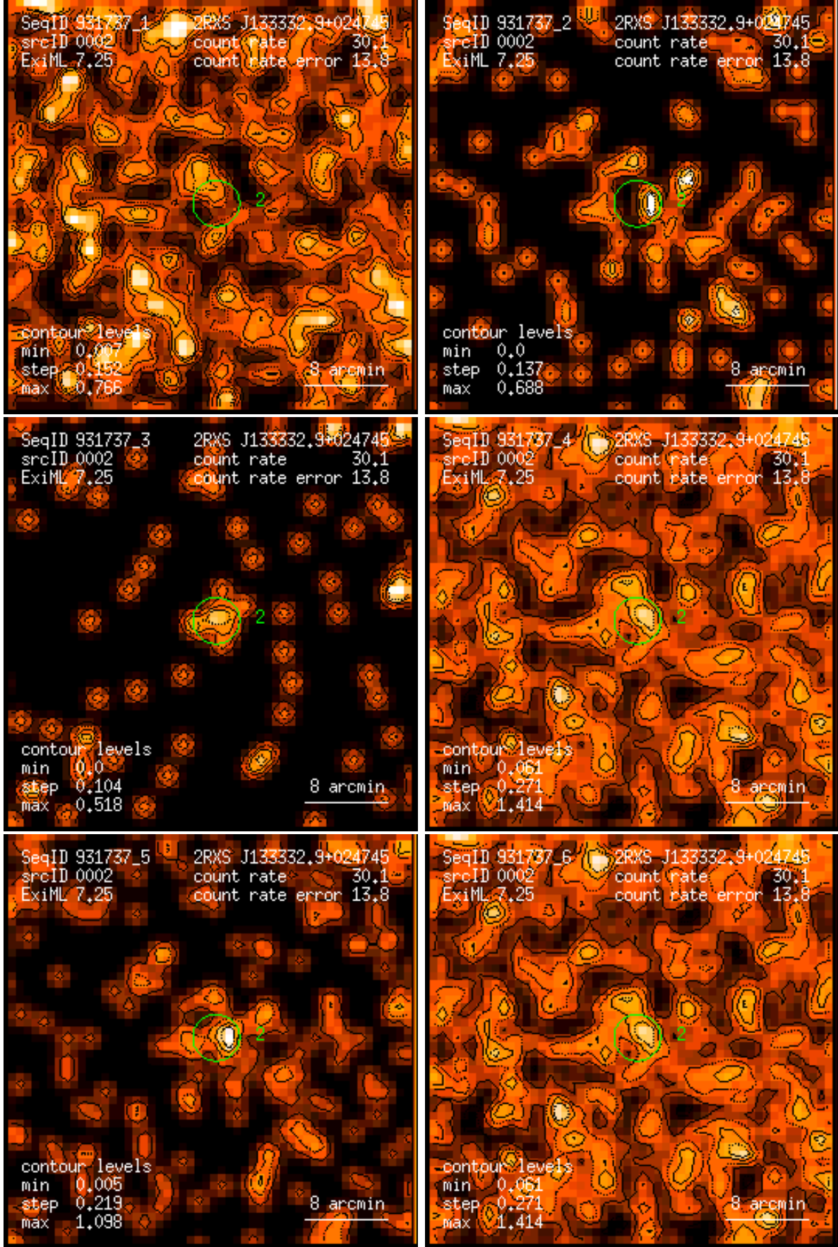
Figure 2: RASS 931737: detection 0002: band rate images, Gaussian filter: (1) PSPC channels 11 – 41, (2) 52 – 90, (3) 91 – 201, (4) 11 – 235, (5) 52 – 201, (6) 11 – 201. Broad band rates in counts/ks. Band rate contour levels in counts/ks/arcmin 2 .
