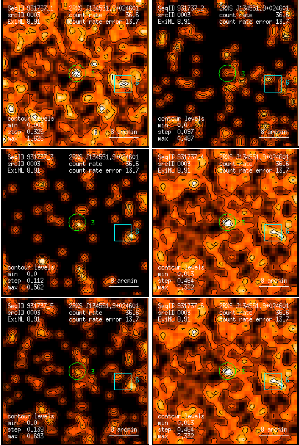
Figure 3: RASS 931737: detection 0003: band rate images, Gaussian filter: (1) PSPC channels 11 – 41, (2) 52 – 90, (3) 91 – 201, (4) 11 – 235, (5) 52 – 201, (6) 11 – 201. Broad band rates in counts/ks. Band rate contour levels in counts/ks/arcmin 2 .
