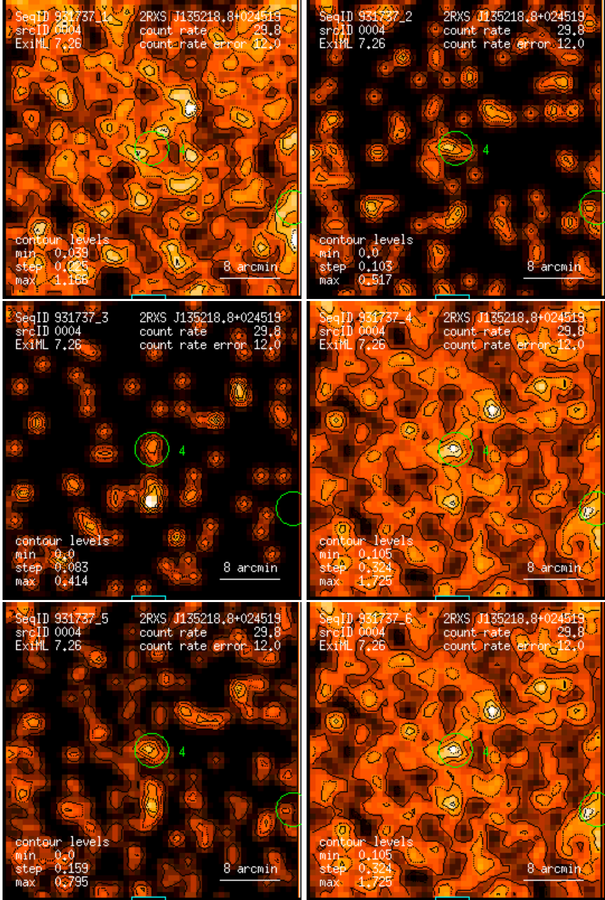
Figure 4: RASS 931737: detection 0004: band rate images, Gaussian filter: (1) PSPC channels 11 – 41, (2) 52 – 90, (3) 91 – 201, (4) 11 – 235, (5) 52 – 201, (6) 11 – 201. Broad band rates in counts/ks. Band rate contour levels in counts/ks/arcmin 2 .
