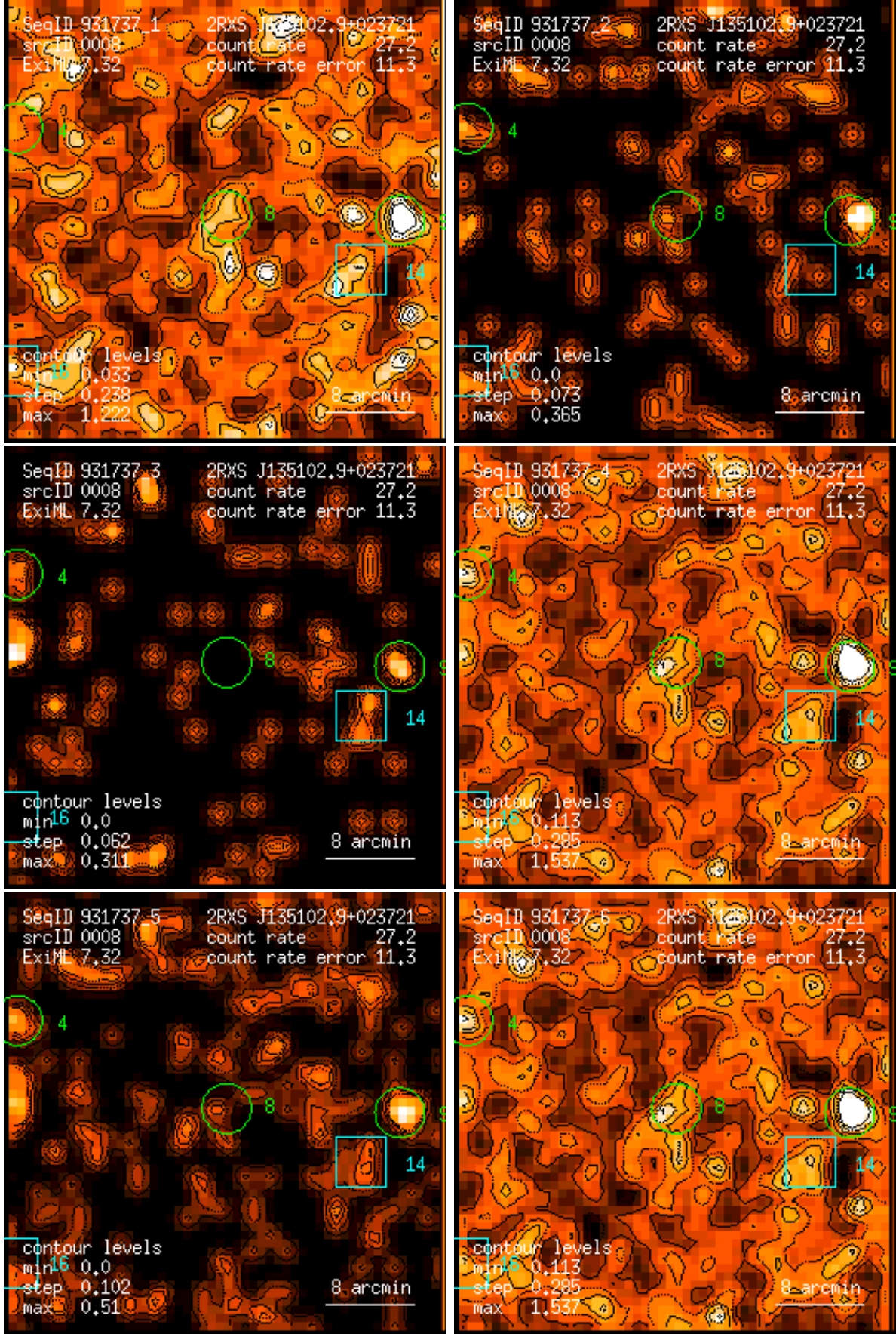
Figure 8: RASS 931737: detection 0008: band rate images, Gaussian filter: (1) PSPC channels 11 – 41, (2) 52 – 90, (3) 91 – 201, (4) 11 – 235, (5) 52 – 201, (6) 11 – 201. Broad band rates in counts/ks. Band rate contour levels in counts/ks/arcmin 2 .
