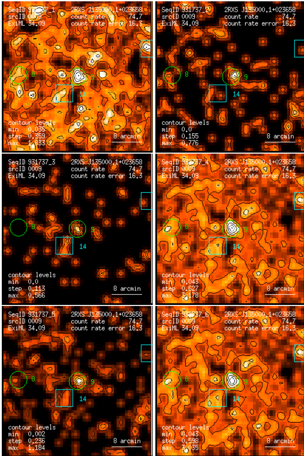
Figure 9: RASS 931737: detection 0009: band rate images, Gaussian filter: (1) PSPC channels 11 – 41, (2) 52 – 90, (3) 91 – 201, (4) 11 – 235, (5) 52 – 201, (6) 11 – 201. Broad band rates in counts/ks. Band rate contour levels in counts/ks/arcmin 2 .
