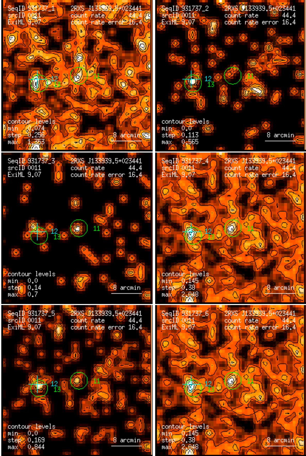
Figure 11: RASS 931737: detection 0011: band rate images, Gaussian filter: (1) PSPC channels 11 – 41, (2) 52 – 90, (3) 91 – 201, (4) 11 – 235, (5) 52 – 201, (6) 11 – 201. Broad band rates in counts/ks. Band rate contour levels in counts/ks/arcmin 2 .
