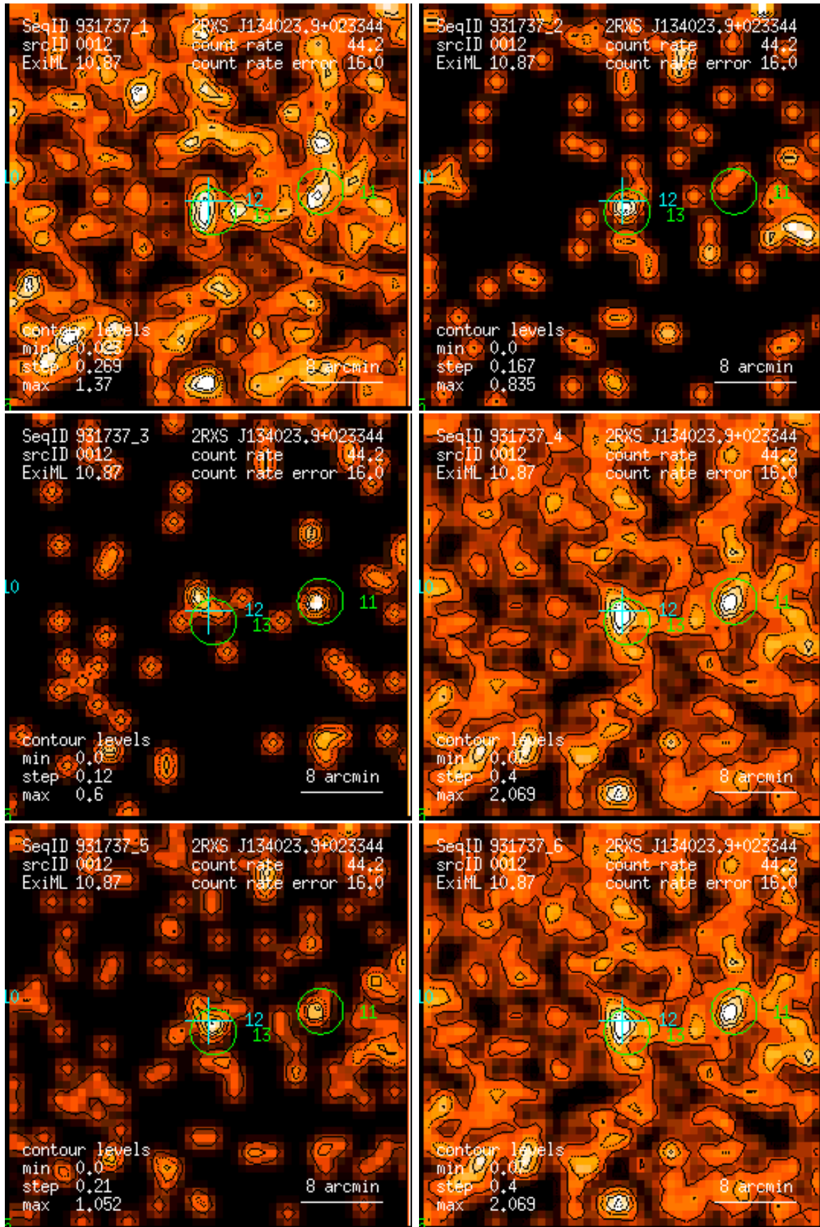
Figure 12: RASS 931737: detection 0012: band rate images, Gaussian filter: (1) PSPC channels 11 – 41, (2) 52 – 90, (3) 91 – 201, (4) 11 – 235, (5) 52 – 201, (6) 11 – 201. Broad band rates in counts/ks. Band rate contour levels in counts/ks/arcmin 2 .
