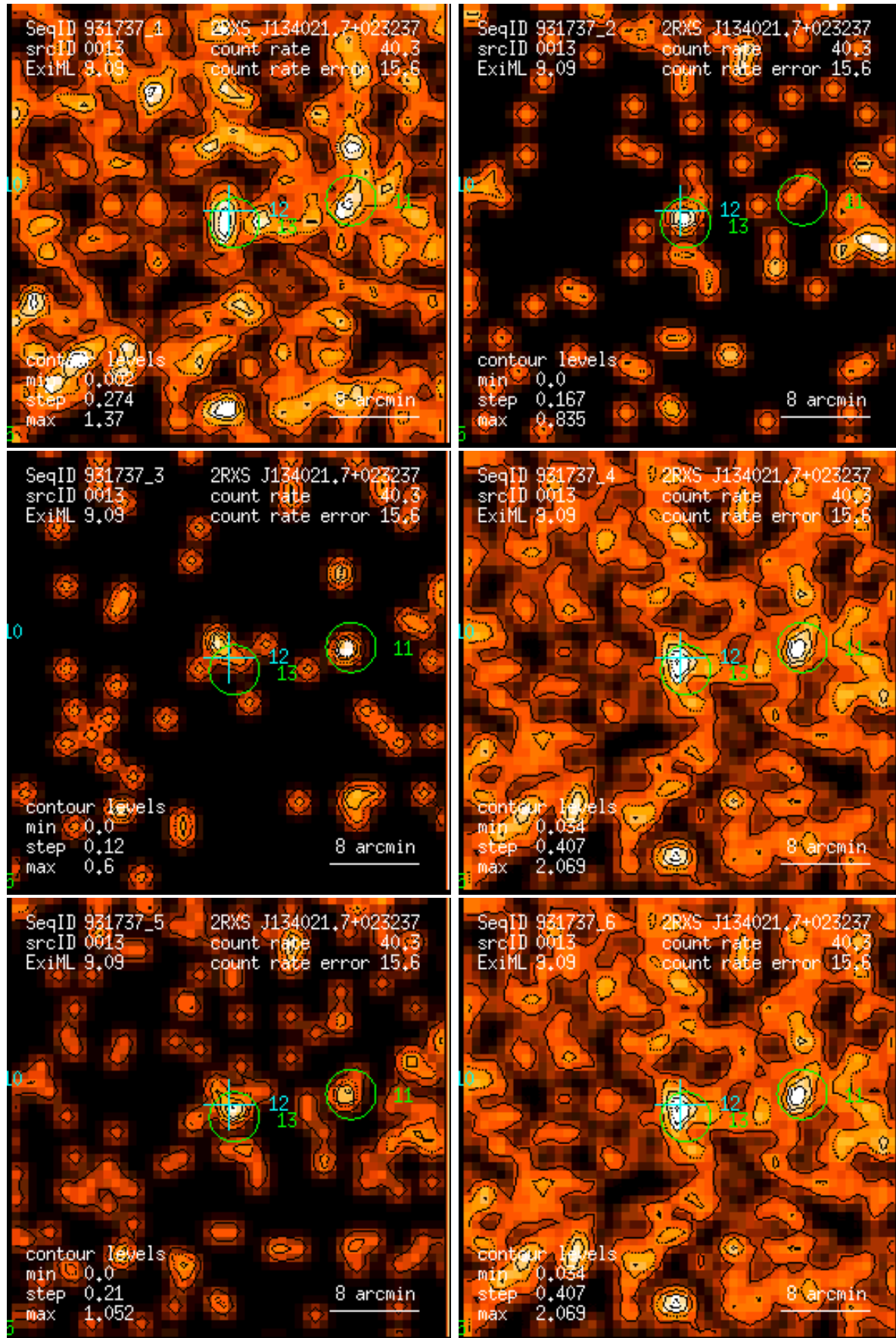
Figure 13: RASS 931737: detection 0013: band rate images, Gaussian filter: (1) PSPC channels 11 – 41, (2) 52 – 90, (3) 91 – 201, (4) 11 – 235, (5) 52 – 201, (6) 11 – 201. Broad band rates in counts/ks. Band rate contour levels in counts/ks/arcmin 2 .
