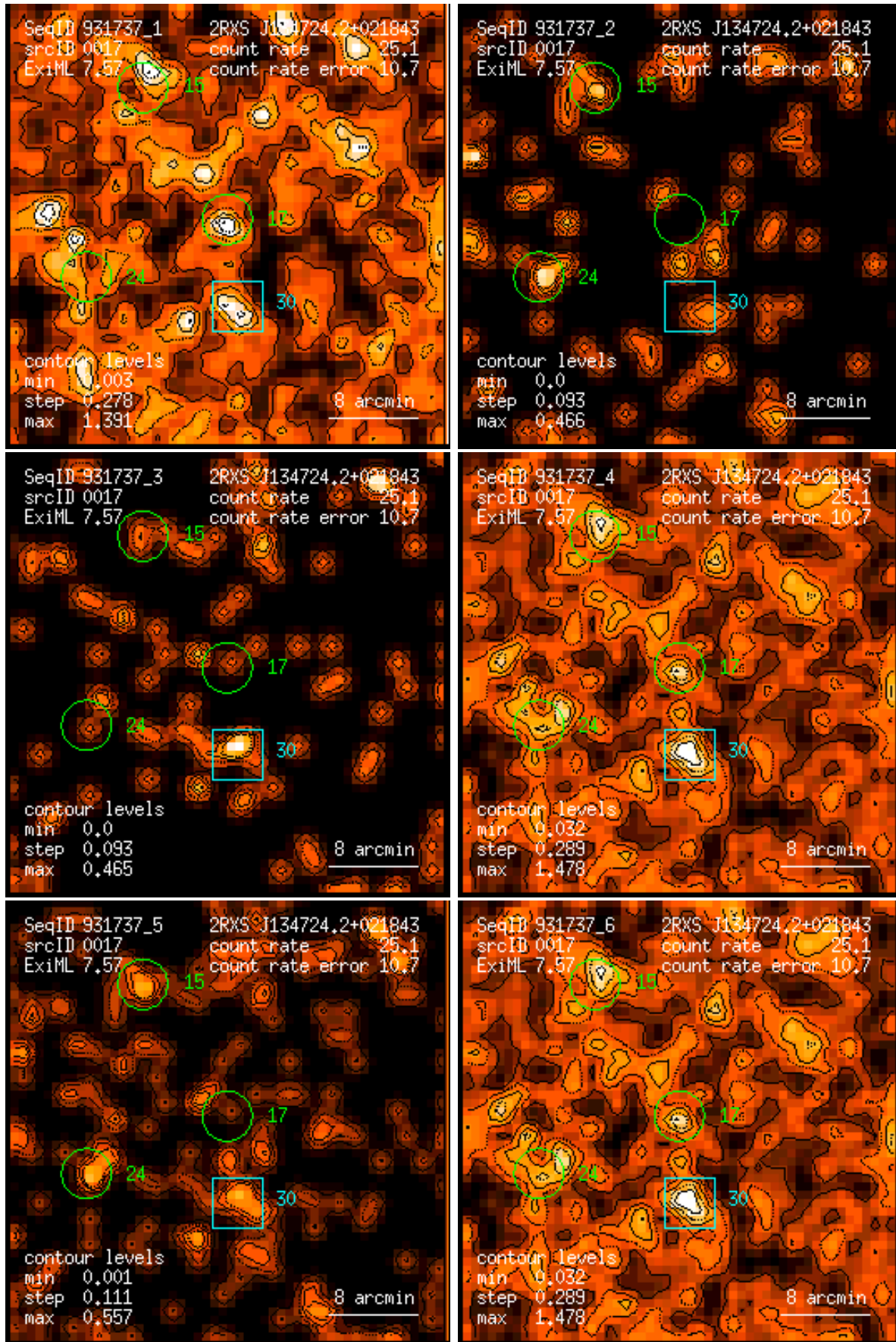
Figure 17: RASS 931737: detection 0017: band rate images, Gaussian filter: (1) PSPC channels 11 – 41, (2) 52 – 90, (3) 91 – 201, (4) 11 – 235, (5) 52 – 201, (6) 11 – 201. Broad band rates in counts/ks. Band rate contour levels in counts/ks/arcmin 2 .
