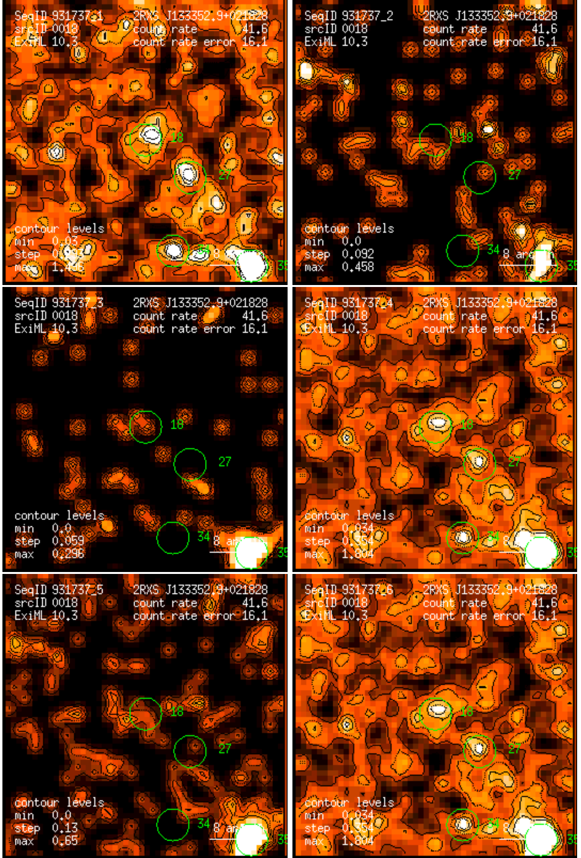
Figure 18: RASS 931737: detection 0018: band rate images, Gaussian filter: (1) PSPC channels 11 – 41, (2) 52 – 90, (3) 91 – 201, (4) 11 – 235, (5) 52 – 201, (6) 11 – 201. Broad band rates in counts/ks. Band rate contour levels in counts/ks/arcmin 2 .
