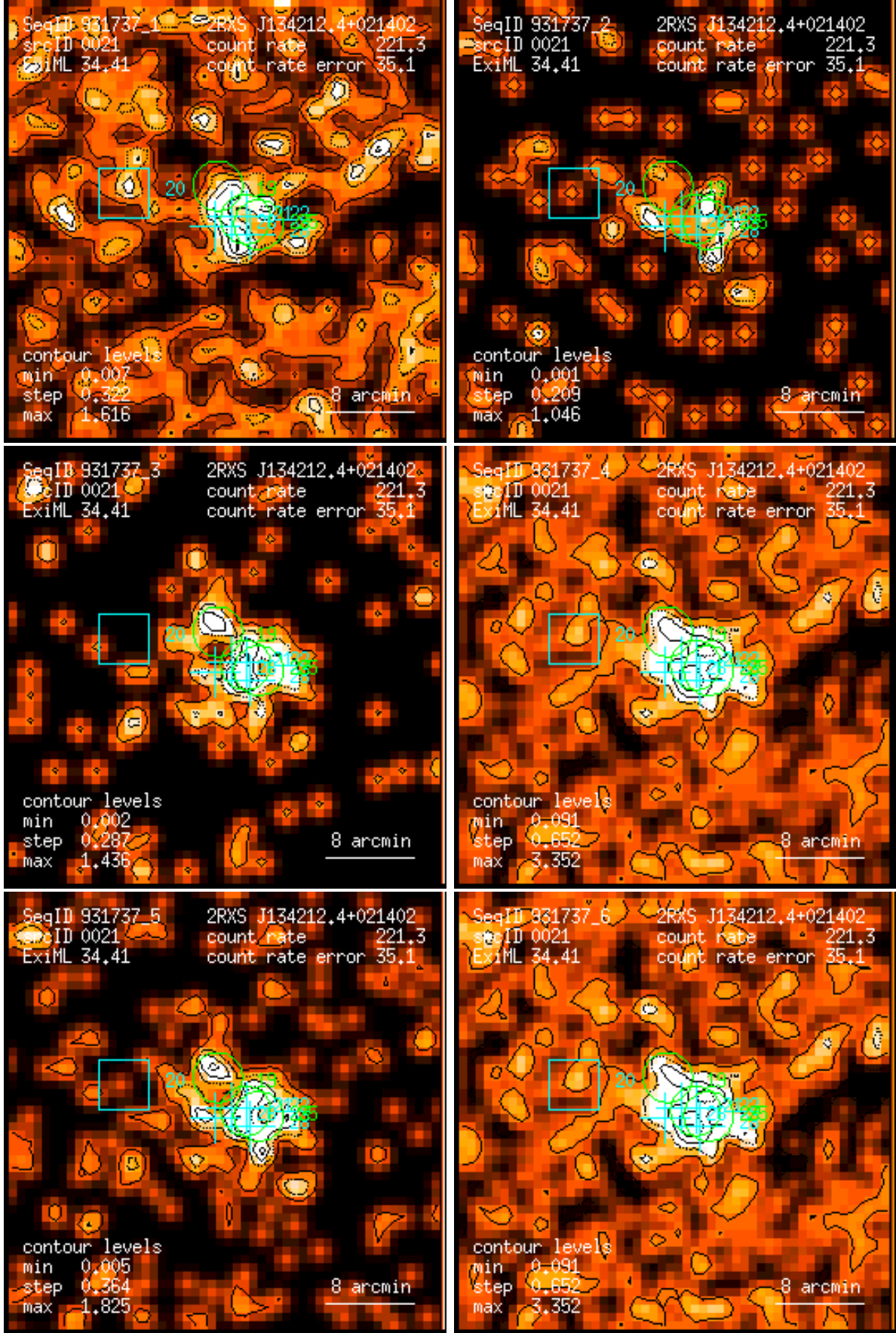
Figure 21: RASS 931737: detection 0021: band rate images, Gaussian filter: (1) PSPC channels 11 – 41, (2) 52 – 90, (3) 91 – 201, (4) 11 – 235, (5) 52 – 201, (6) 11 – 201. Broad band rates in counts/ks. Band rate contour levels in counts/ks/arcmin 2 .
