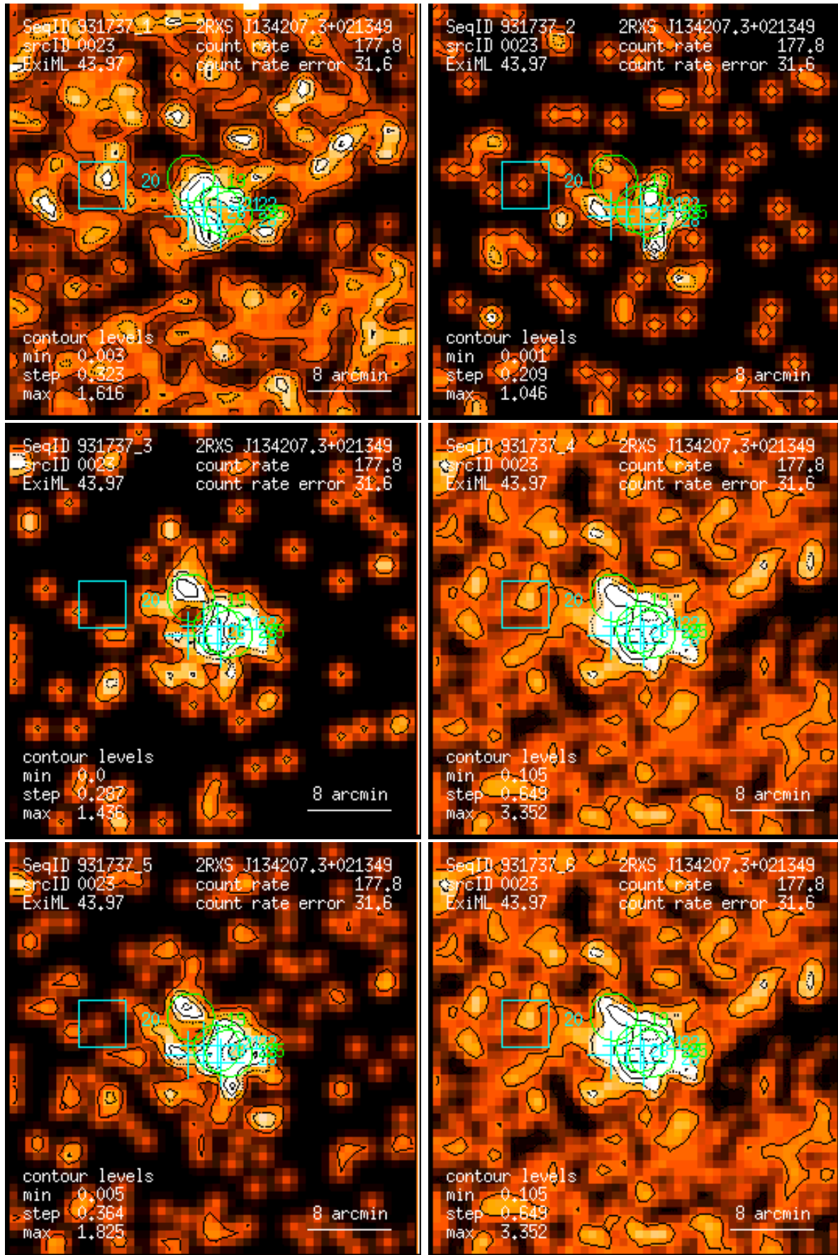
Figure 23: RASS 931737: detection 0023: band rate images, Gaussian filter: (1) PSPC channels 11 – 41, (2) 52 – 90, (3) 91 – 201, (4) 11 – 235, (5) 52 – 201, (6) 11 – 201. Broad band rates in counts/ks. Band rate contour levels in counts/ks/arcmin 2 .
