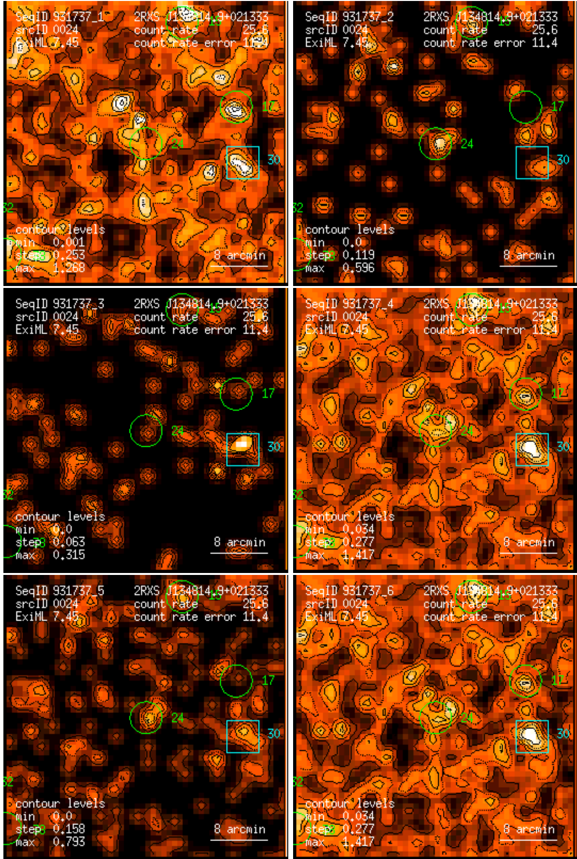
Figure 24: RASS 931737: detection 0024: band rate images, Gaussian filter: (1) PSPC channels 11 – 41, (2) 52 – 90, (3) 91 – 201, (4) 11 – 235, (5) 52 – 201, (6) 11 – 201. Broad band rates in counts/ks. Band rate contour levels in counts/ks/arcmin 2 .
