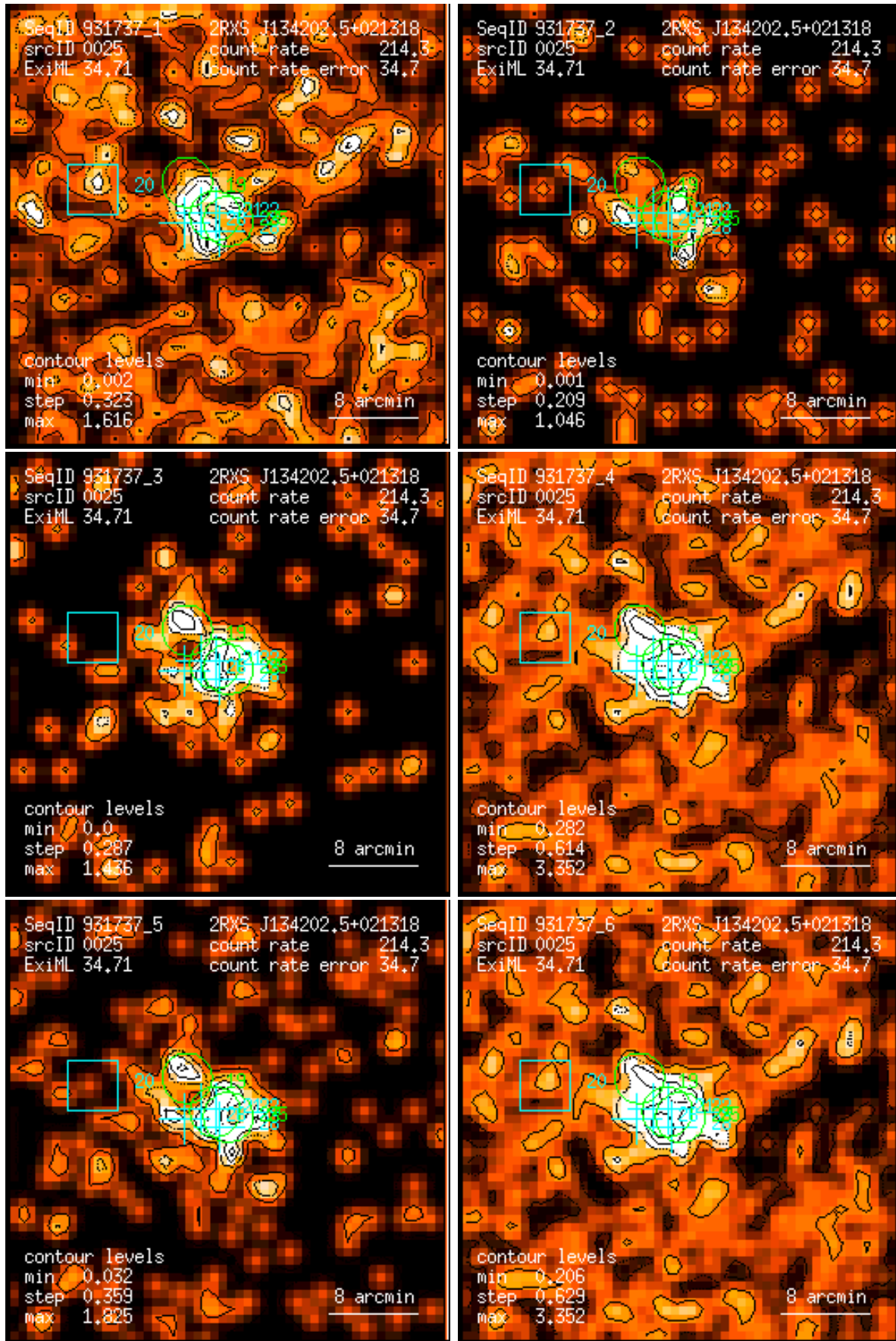
Figure 25: RASS 931737: detection 0025: band rate images, Gaussian filter: (1) PSPC channels 11 – 41, (2) 52 – 90, (3) 91 – 201, (4) 11 – 235, (5) 52 – 201, (6) 11 – 201. Broad band rates in counts/ks. Band rate contour levels in counts/ks/arcmin 2 .
