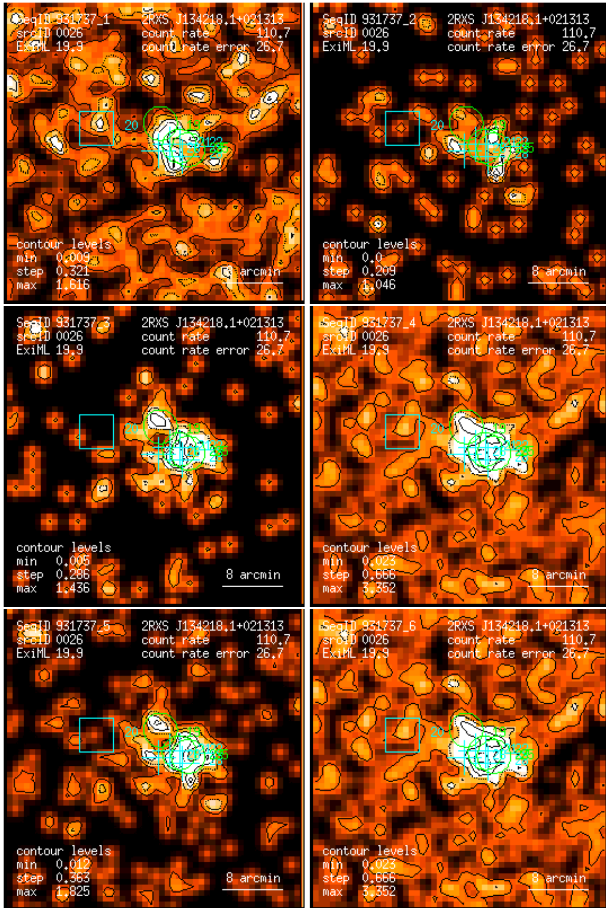
Figure 26: RASS 931737: detection 0026: band rate images, Gaussian filter: (1) PSPC channels 11 – 41, (2) 52 – 90, (3) 91 – 201, (4) 11 – 235, (5) 52 – 201, (6) 11 – 201. Broad band rates in counts/ks. Band rate contour levels in counts/ks/arcmin 2 .
