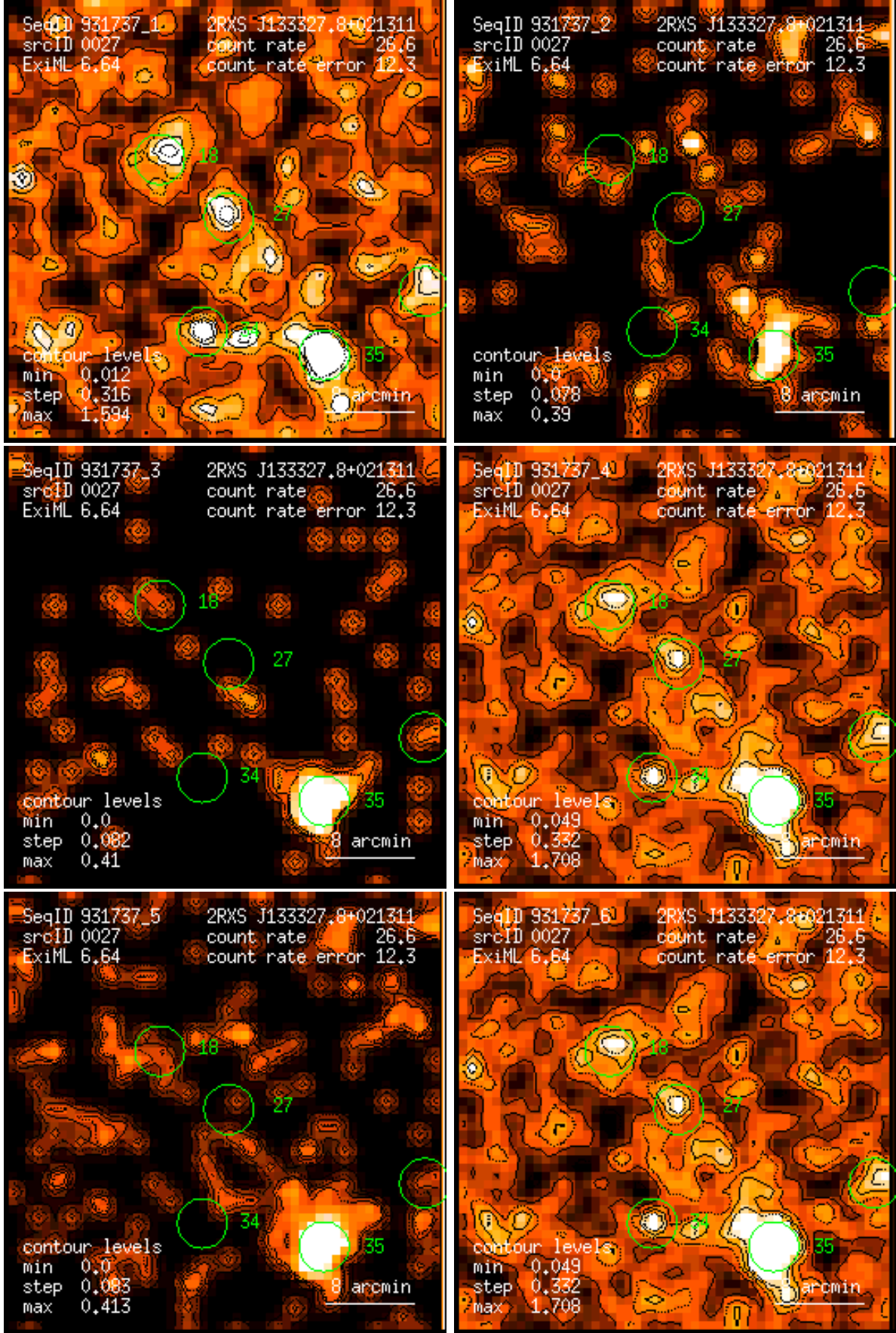
Figure 27: RASS 931737: detection 0027: band rate images, Gaussian filter: (1) PSPC channels 11 – 41, (2) 52 – 90, (3) 91 – 201, (4) 11 – 235, (5) 52 – 201, (6) 11 – 201. Broad band rates in counts/ks. Band rate contour levels in counts/ks/arcmin 2 .
