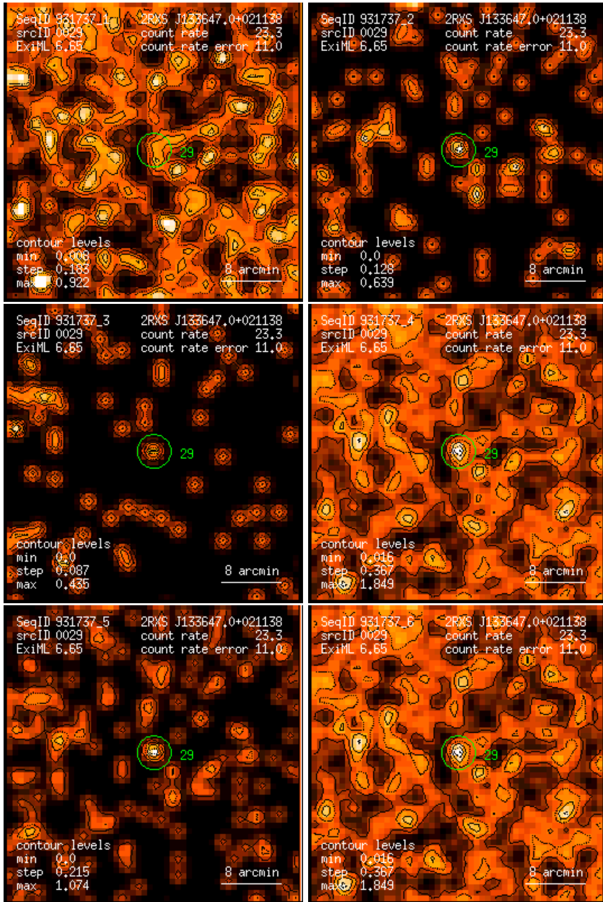
Figure 29: RASS 931737: detection 0029: band rate images, Gaussian filter: (1) PSPC channels 11 – 41, (2) 52 – 90, (3) 91 – 201, (4) 11 – 235, (5) 52 – 201, (6) 11 – 201. Broad band rates in counts/ks. Band rate contour levels in counts/ks/arcmin 2 .
