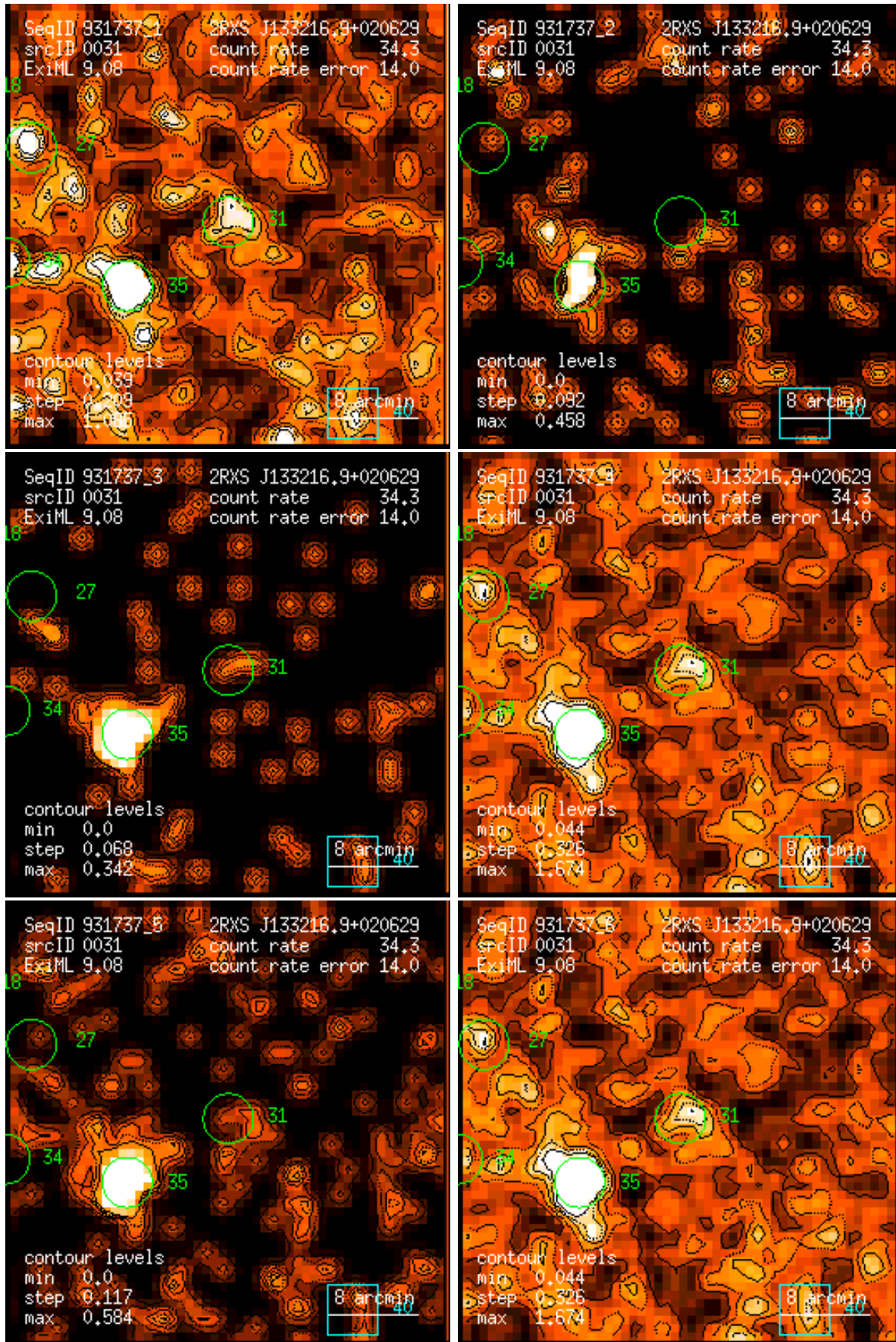
Figure 31: RASS 931737: detection 0031: band rate images, Gaussian filter: (1) PSPC channels 11 – 41, (2) 52 – 90, (3) 91 – 201, (4) 11 – 235, (5) 52 – 201, (6) 11 – 201. Broad band rates in counts/ks. Band rate contour levels in counts/ks/arcmin 2 .
