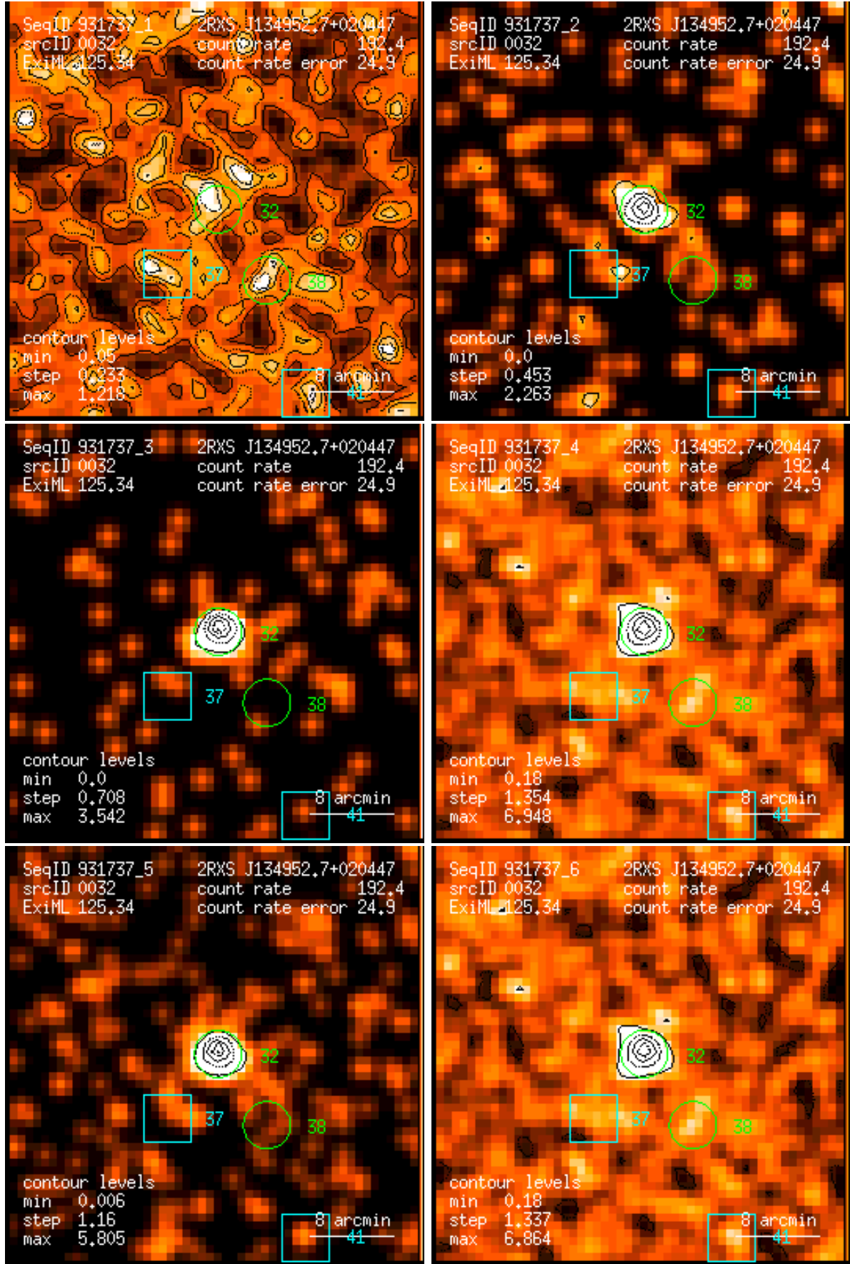
Figure 32: RASS 931737: detection 0032: band rate images, Gaussian filter: (1) PSPC channels 11 – 41, (2) 52 – 90, (3) 91 – 201, (4) 11 – 235, (5) 52 – 201, (6) 11 – 201. Broad band rates in counts/ks. Band rate contour levels in counts/ks/arcmin 2 .
