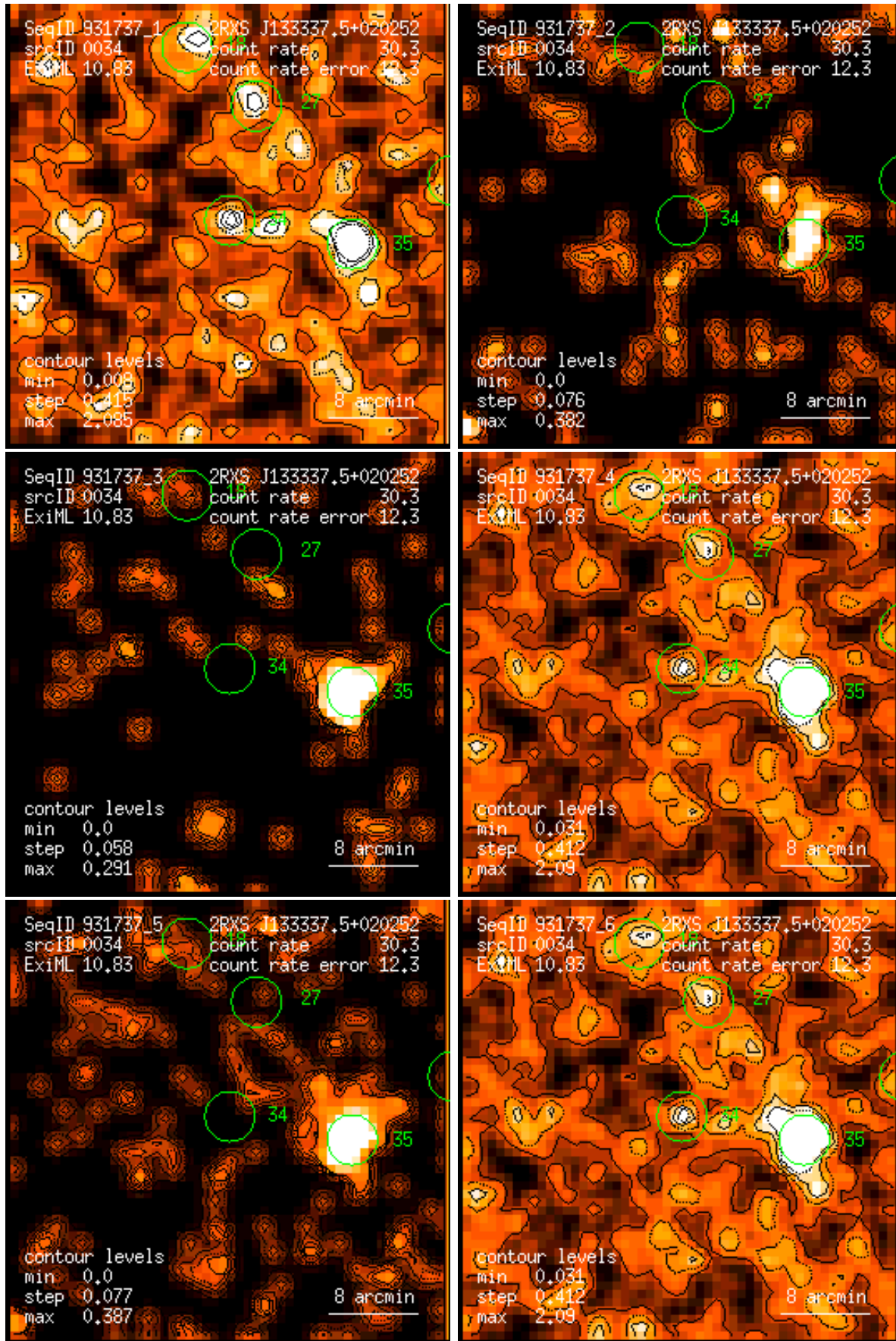
Figure 34: RASS 931737: detection 0034: band rate images, Gaussian filter: (1) PSPC channels 11 – 41, (2) 52 – 90, (3) 91 – 201, (4) 11 – 235, (5) 52 – 201, (6) 11 – 201. Broad band rates in counts/ks. Band rate contour levels in counts/ks/arcmin 2 .
