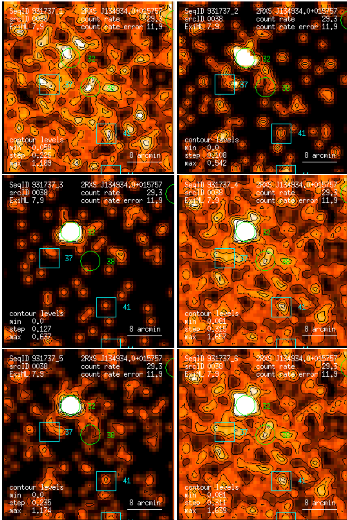
Figure 38: RASS 931737: detection 0038: band rate images, Gaussian filter: (1) PSPC channels 11 – 41, (2) 52 – 90, (3) 91 – 201, (4) 11 – 235, (5) 52 – 201, (6) 11 – 201. Broad band rates in counts/ks. Band rate contour levels in counts/ks/arcmin 2 .
