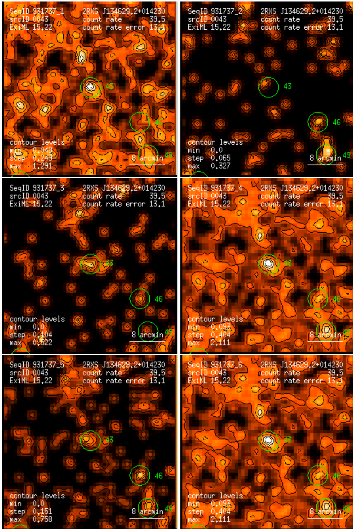
Figure 43: RASS 931737: detection 0043: band rate images, Gaussian filter: (1) PSPC channels 11 – 41, (2) 52 – 90, (3) 91 – 201, (4) 11 – 235, (5) 52 – 201, (6) 11 – 201. Broad band rates in counts/ks. Band rate contour levels in counts/ks/arcmin 2 .
