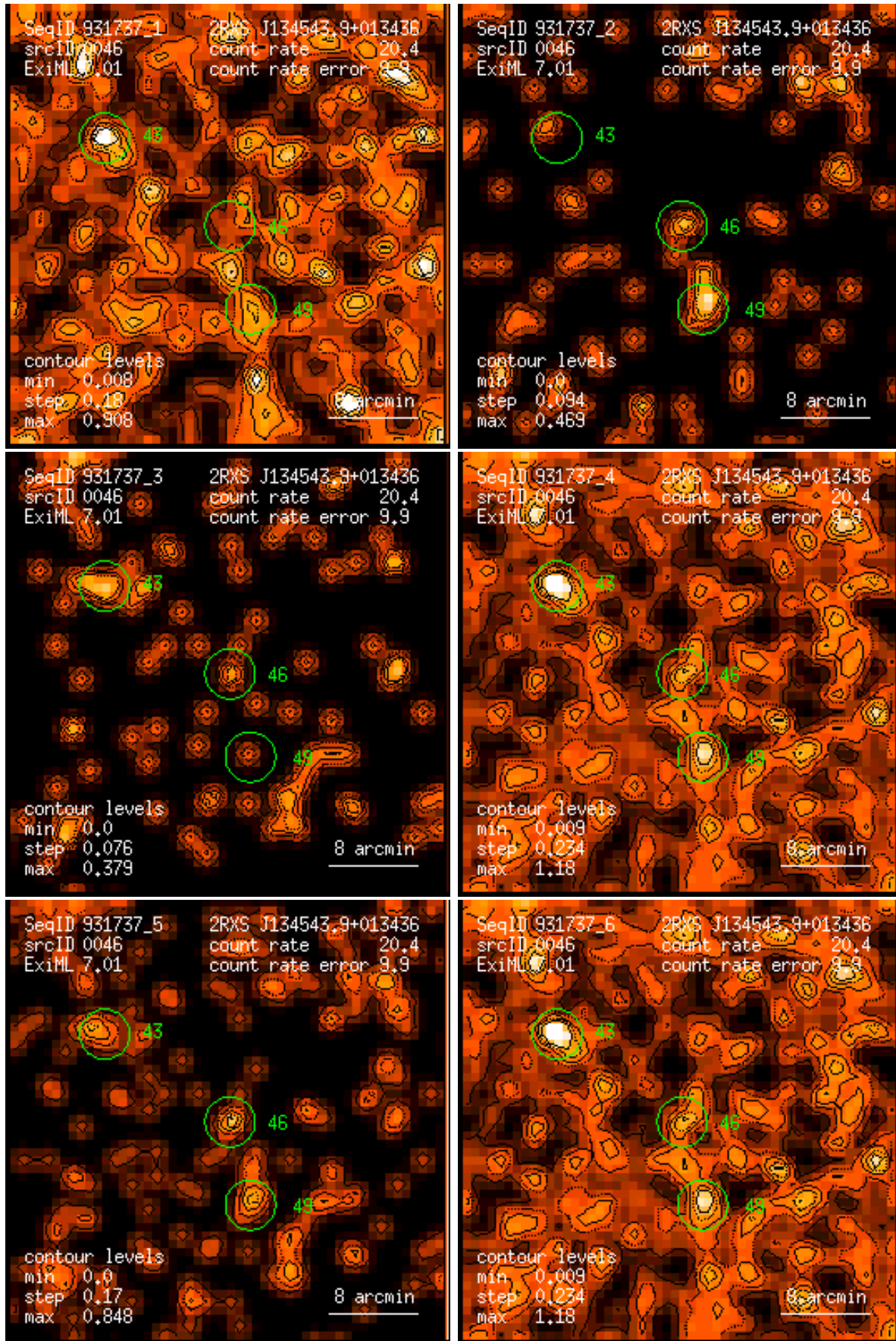
Figure 46: RASS 931737: detection 0046: band rate images, Gaussian filter: (1) PSPC channels 11 – 41, (2) 52 – 90, (3) 91 – 201, (4) 11 – 235, (5) 52 – 201, (6) 11 – 201. Broad band rates in counts/ks. Band rate contour levels in counts/ks/arcmin 2 .
