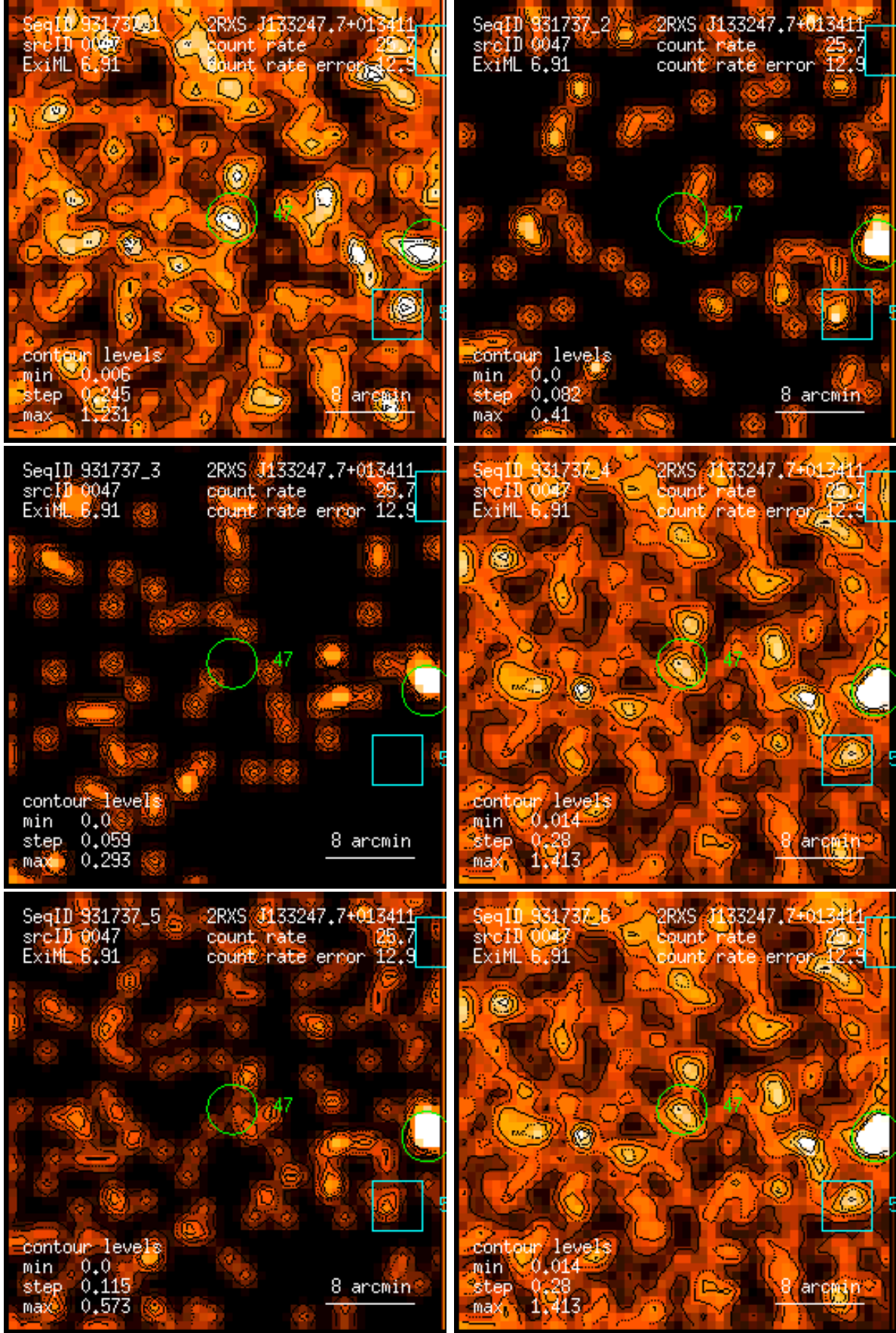
Figure 47: RASS 931737: detection 0047: band rate images, Gaussian filter: (1) PSPC channels 11 – 41, (2) 52 – 90, (3) 91 – 201, (4) 11 – 235, (5) 52 – 201, (6) 11 – 201. Broad band rates in counts/ks. Band rate contour levels in counts/ks/arcmin 2 .
