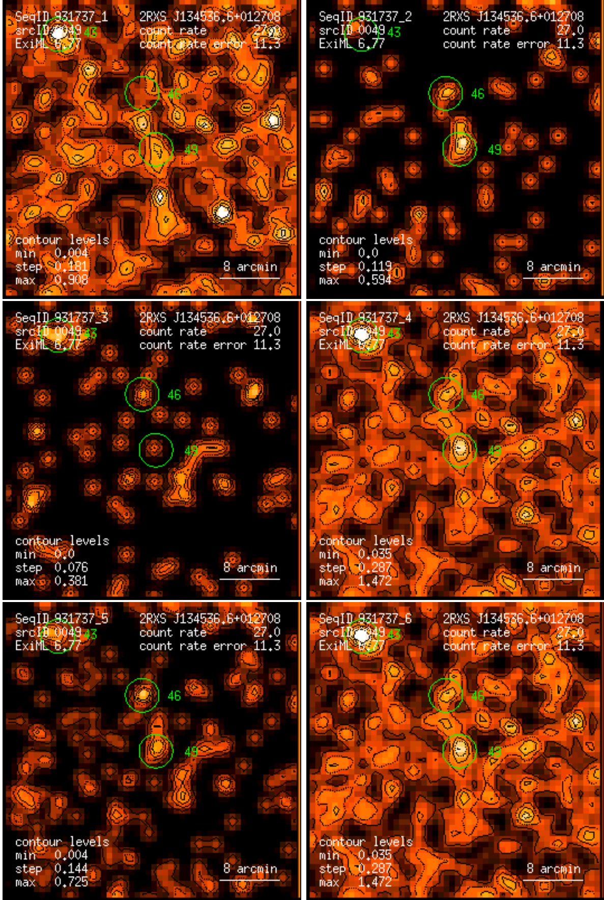
Figure 49: RASS 931737: detection 0049: band rate images, Gaussian filter: (1) PSPC channels 11 – 41, (2) 52 – 90, (3) 91 – 201, (4) 11 – 235, (5) 52 – 201, (6) 11 – 201. Broad band rates in counts/ks. Band rate contour levels in counts/ks/arcmin 2 .
