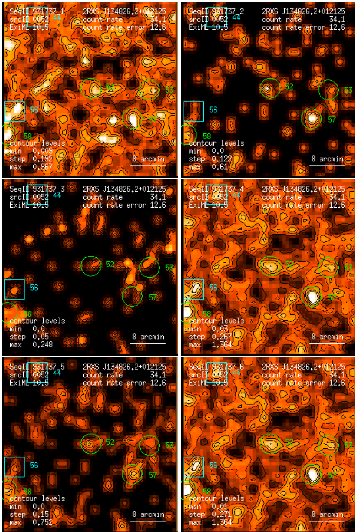
Figure 52: RASS 931737: detection 0052: band rate images, Gaussian filter: (1) PSPC channels 11 – 41, (2) 52 – 90, (3) 91 – 201, (4) 11 – 235, (5) 52 – 201, (6) 11 – 201. Broad band rates in counts/ks. Band rate contour levels in counts/ks/arcmin 2 .
