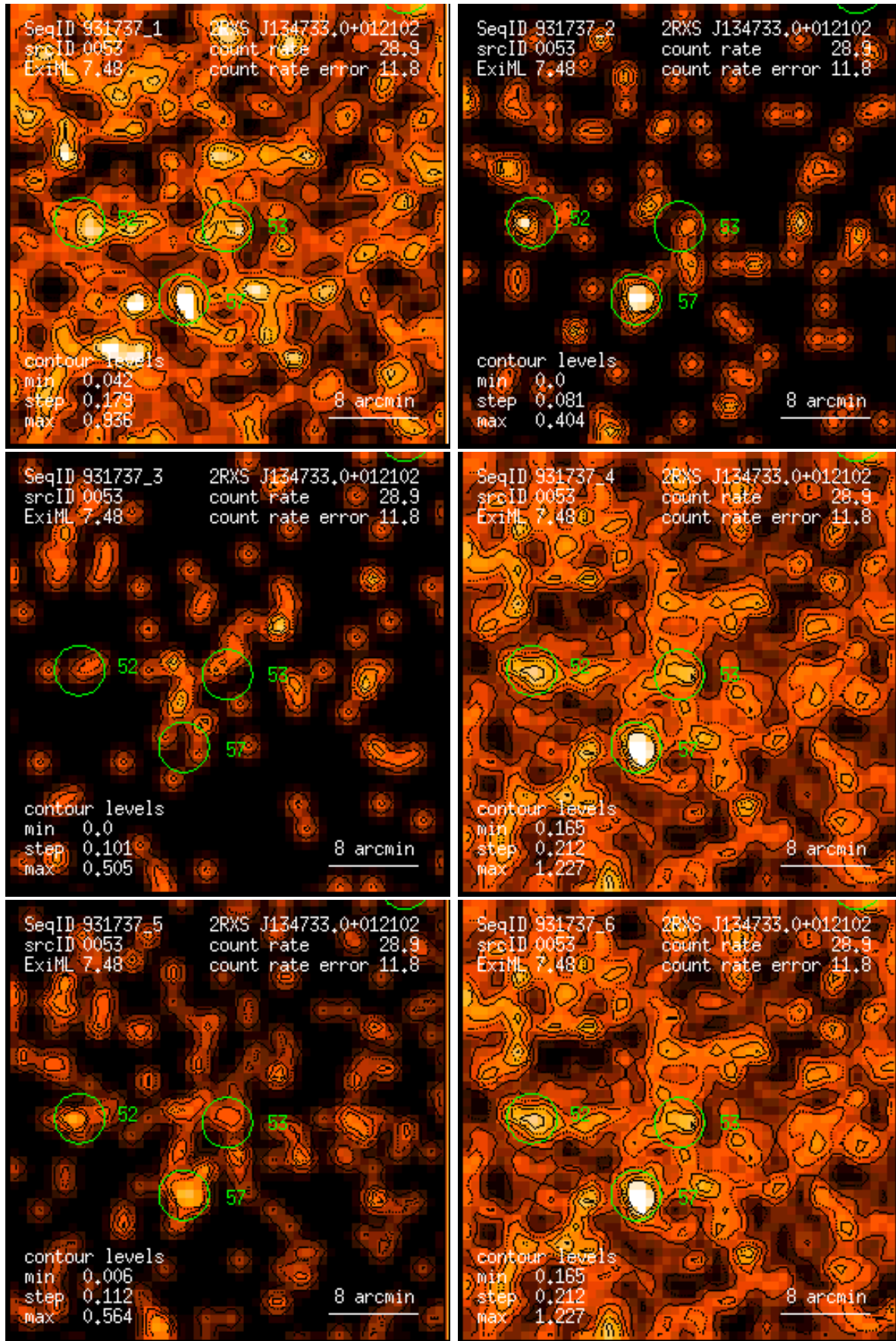
Figure 53: RASS 931737: detection 0053: band rate images, Gaussian filter: (1) PSPC channels 11 – 41, (2) 52 – 90, (3) 91 – 201, (4) 11 – 235, (5) 52 – 201, (6) 11 – 201. Broad band rates in counts/ks. Band rate contour levels in counts/ks/arcmin 2 .
