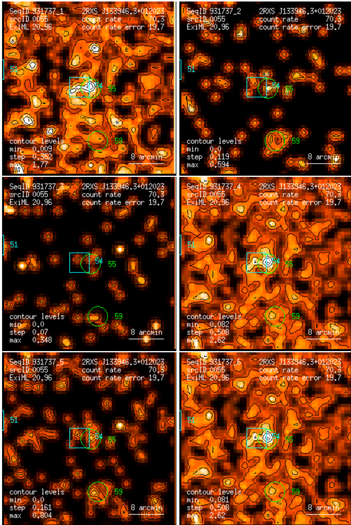
Figure 55: RASS 931737: detection 0055: band rate images, Gaussian filter: (1) PSPC channels 11 – 41, (2) 52 – 90, (3) 91 – 201, (4) 11 – 235, (5) 52 – 201, (6) 11 – 201. Broad band rates in counts/ks. Band rate contour levels in counts/ks/arcmin 2 .
