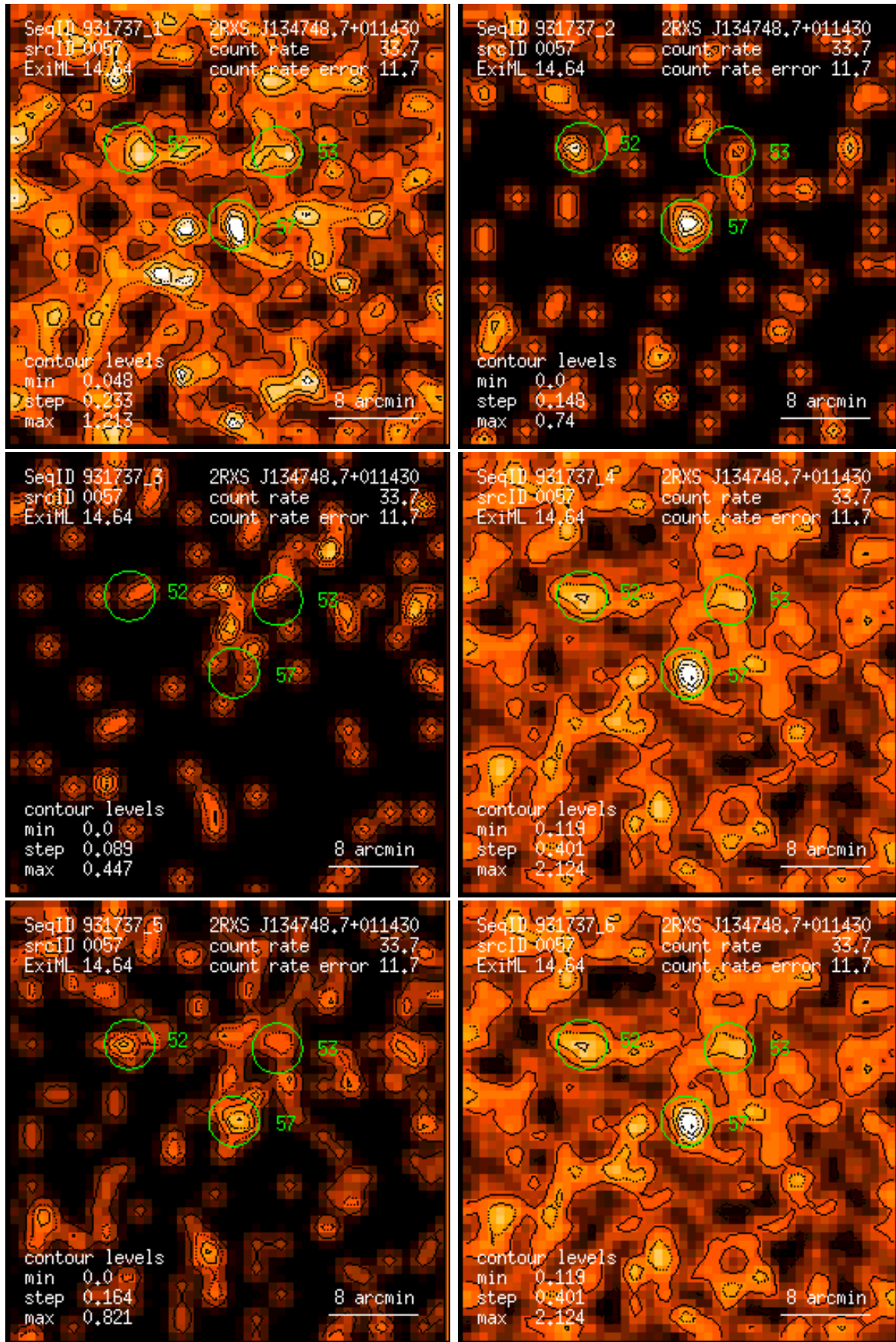
Figure 57: RASS 931737: detection 0057: band rate images, Gaussian filter: (1) PSPC channels 11 – 41, (2) 52 – 90, (3) 91 – 201, (4) 11 – 235, (5) 52 – 201, (6) 11 – 201. Broad band rates in counts/ks. Band rate contour levels in counts/ks/arcmin 2 .
