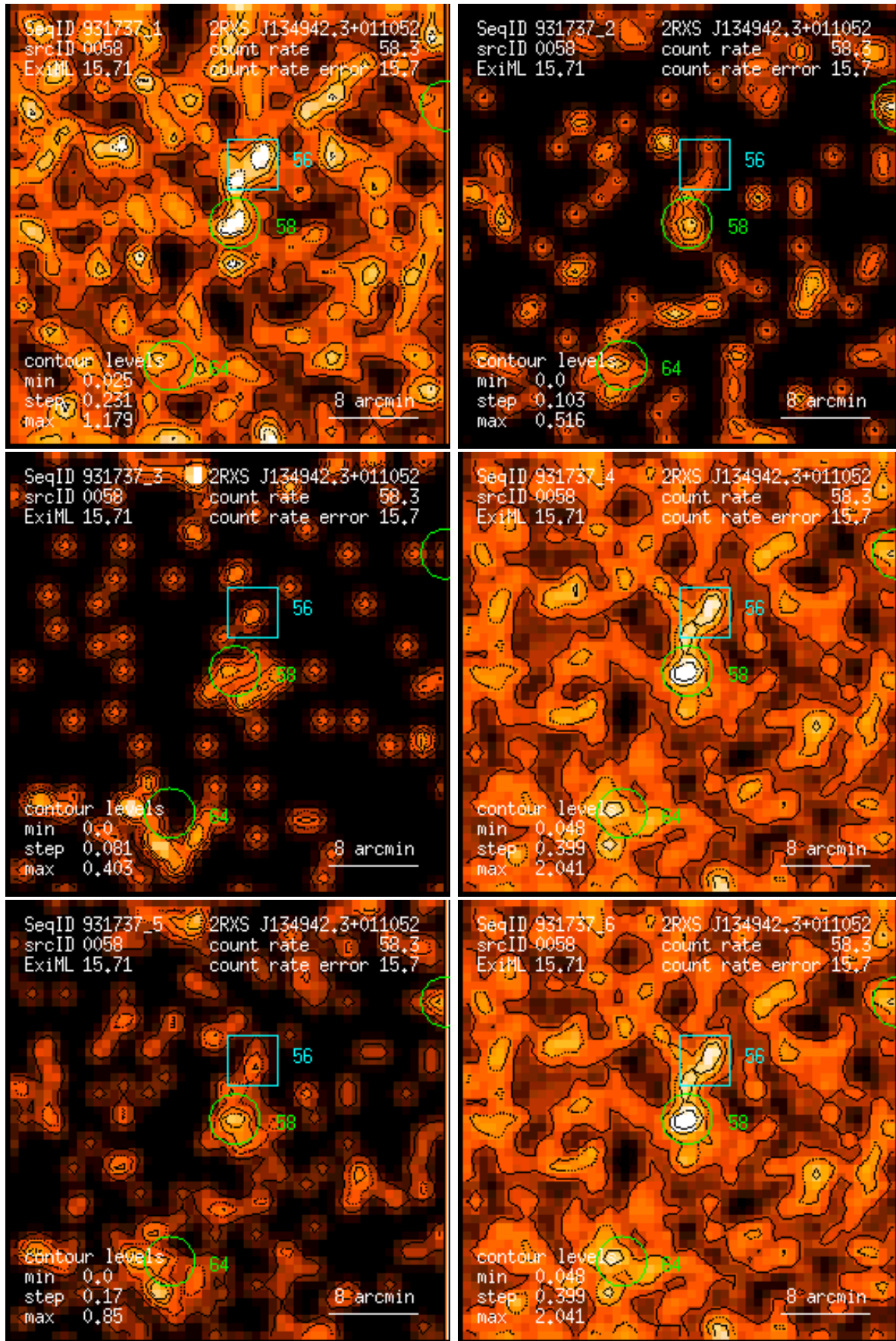
Figure 58: RASS 931737: detection 0058: band rate images, Gaussian filter: (1) PSPC channels 11 – 41, (2) 52 – 90, (3) 91 – 201, (4) 11 – 235, (5) 52 – 201, (6) 11 – 201. Broad band rates in counts/ks. Band rate contour levels in counts/ks/arcmin 2 .
