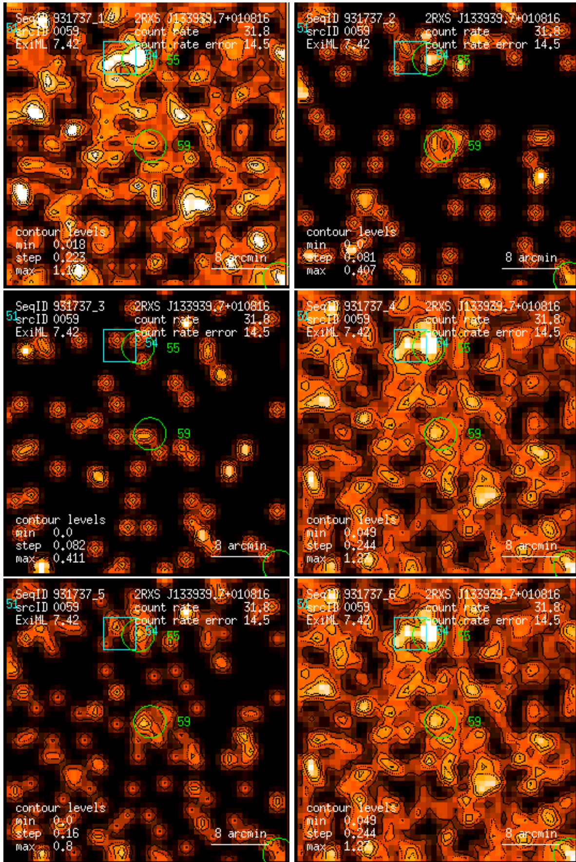
Figure 59: RASS 931737: detection 0059: band rate images, Gaussian filter: (1) PSPC channels 11 – 41, (2) 52 – 90, (3) 91 – 201, (4) 11 – 235, (5) 52 – 201, (6) 11 – 201. Broad band rates in counts/ks. Band rate contour levels in counts/ks/arcmin 2 .
