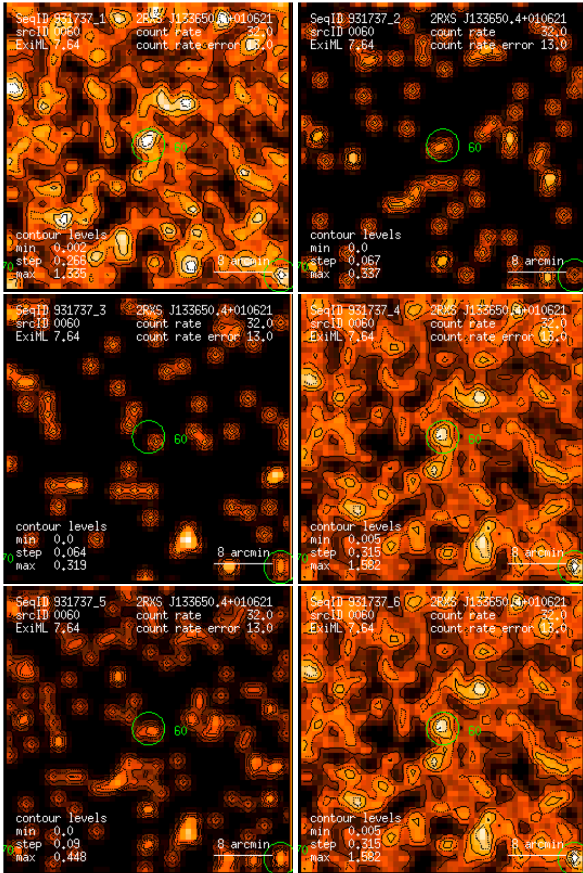
Figure 60: RASS 931737: detection 0060: band rate images, Gaussian filter: (1) PSPC channels 11 – 41, (2) 52 – 90, (3) 91 – 201, (4) 11 – 235, (5) 52 – 201, (6) 11 – 201. Broad band rates in counts/ks. Band rate contour levels in counts/ks/arcmin 2 .
