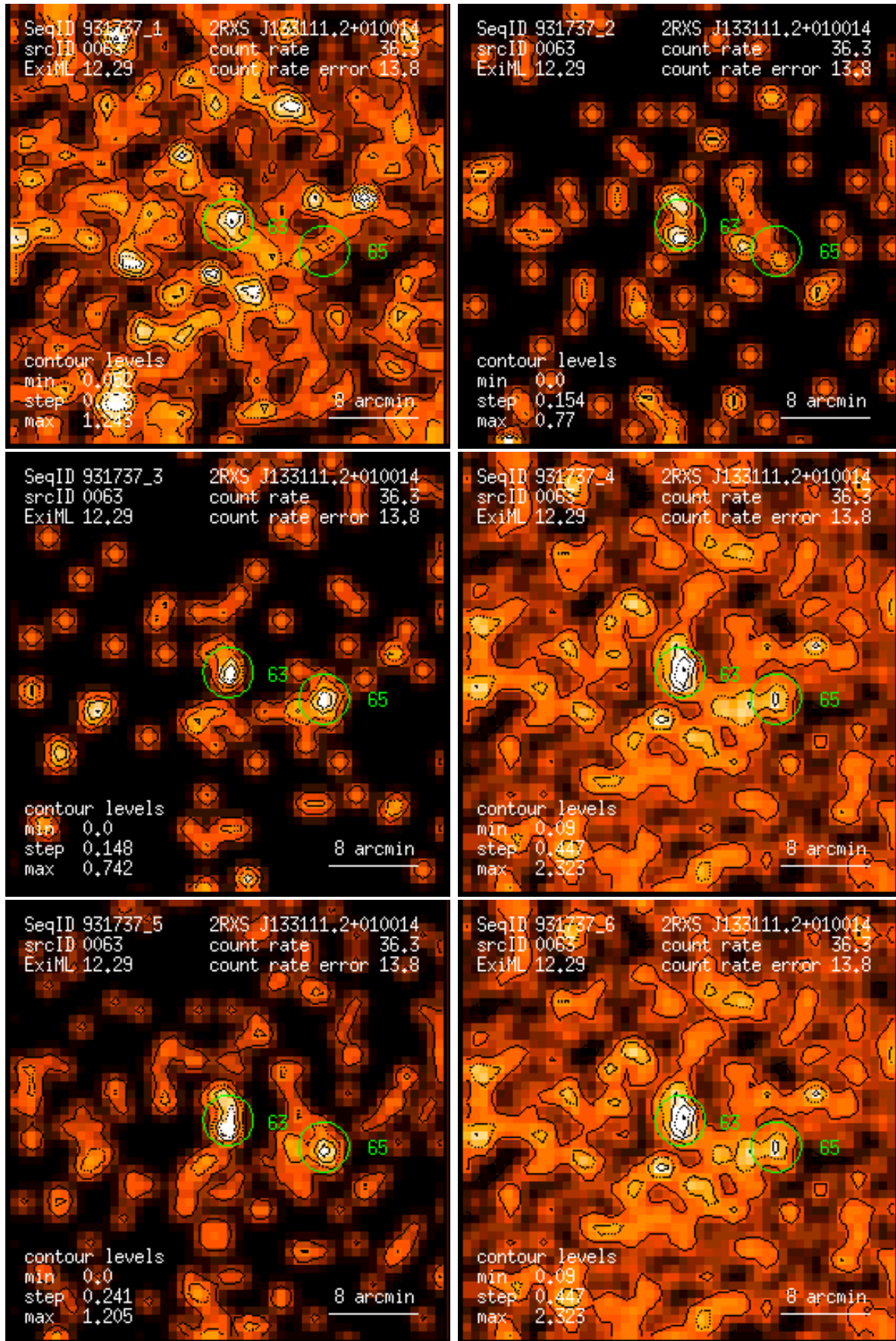
Figure 63: RASS 931737: detection 0063: band rate images, Gaussian filter: (1) PSPC channels 11 – 41, (2) 52 – 90, (3) 91 – 201, (4) 11 – 235, (5) 52 – 201, (6) 11 – 201. Broad band rates in counts/ks. Band rate contour levels in counts/ks/arcmin 2 .
