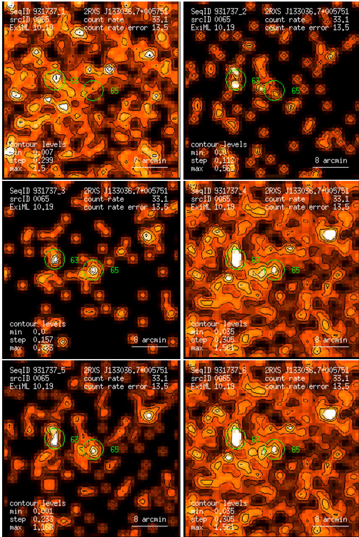
Figure 65: RASS 931737: detection 0065: band rate images, Gaussian filter: (1) PSPC channels 11 – 41, (2) 52 – 90, (3) 91 – 201, (4) 11 – 235, (5) 52 – 201, (6) 11 – 201. Broad band rates in counts/ks. Band rate contour levels in counts/ks/arcmin 2 .
