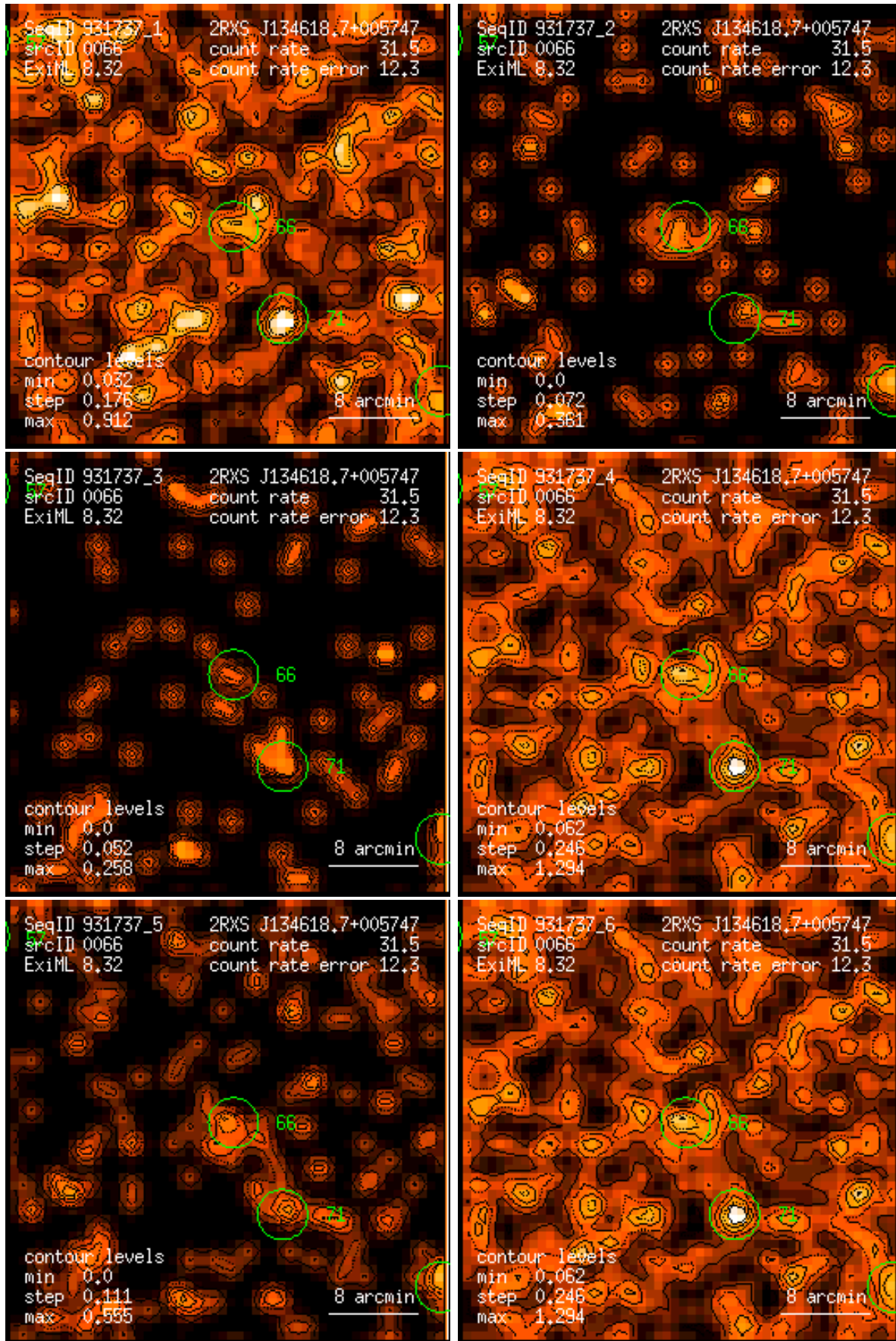
Figure 66: RASS 931737: detection 0066: band rate images, Gaussian filter: (1) PSPC channels 11 – 41, (2) 52 – 90, (3) 91 – 201, (4) 11 – 235, (5) 52 – 201, (6) 11 – 201. Broad band rates in counts/ks. Band rate contour levels in counts/ks/arcmin 2 .
