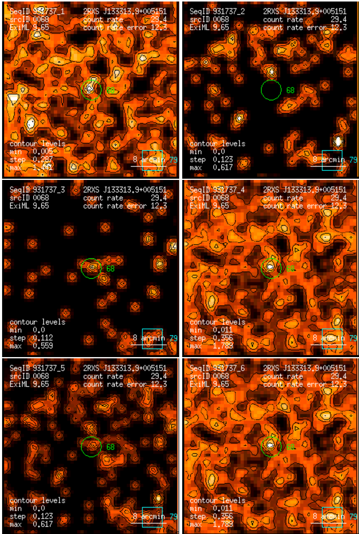
Figure 68: RASS 931737: detection 0068: band rate images, Gaussian filter: (1) PSPC channels 11 – 41, (2) 52 – 90, (3) 91 – 201, (4) 11 – 235, (5) 52 – 201, (6) 11 – 201. Broad band rates in counts/ks. Band rate contour levels in counts/ks/arcmin 2 .
