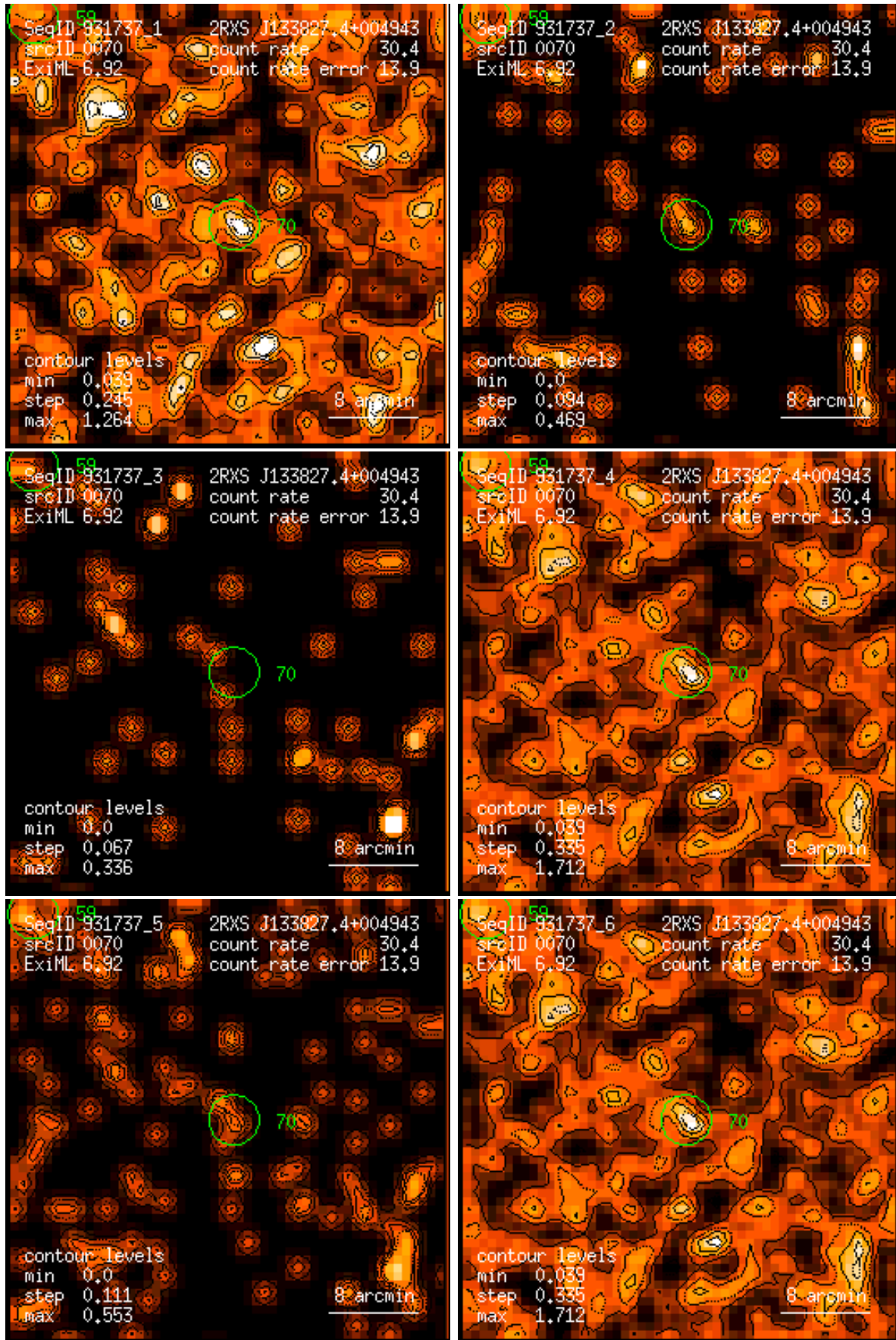
Figure 70: RASS 931737: detection 0070: band rate images, Gaussian filter: (1) PSPC channels 11 – 41, (2) 52 – 90, (3) 91 – 201, (4) 11 – 235, (5) 52 – 201, (6) 11 – 201. Broad band rates in counts/ks. Band rate contour levels in counts/ks/arcmin 2 .
