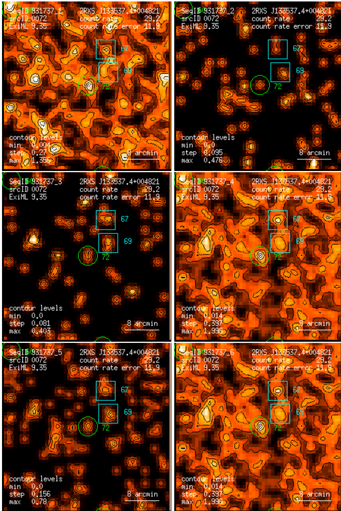
Figure 72: RASS 931737: detection 0072: band rate images, Gaussian filter: (1) PSPC channels 11 – 41, (2) 52 – 90, (3) 91 – 201, (4) 11 – 235, (5) 52 – 201, (6) 11 – 201. Broad band rates in counts/ks. Band rate contour levels in counts/ks/arcmin 2 .
