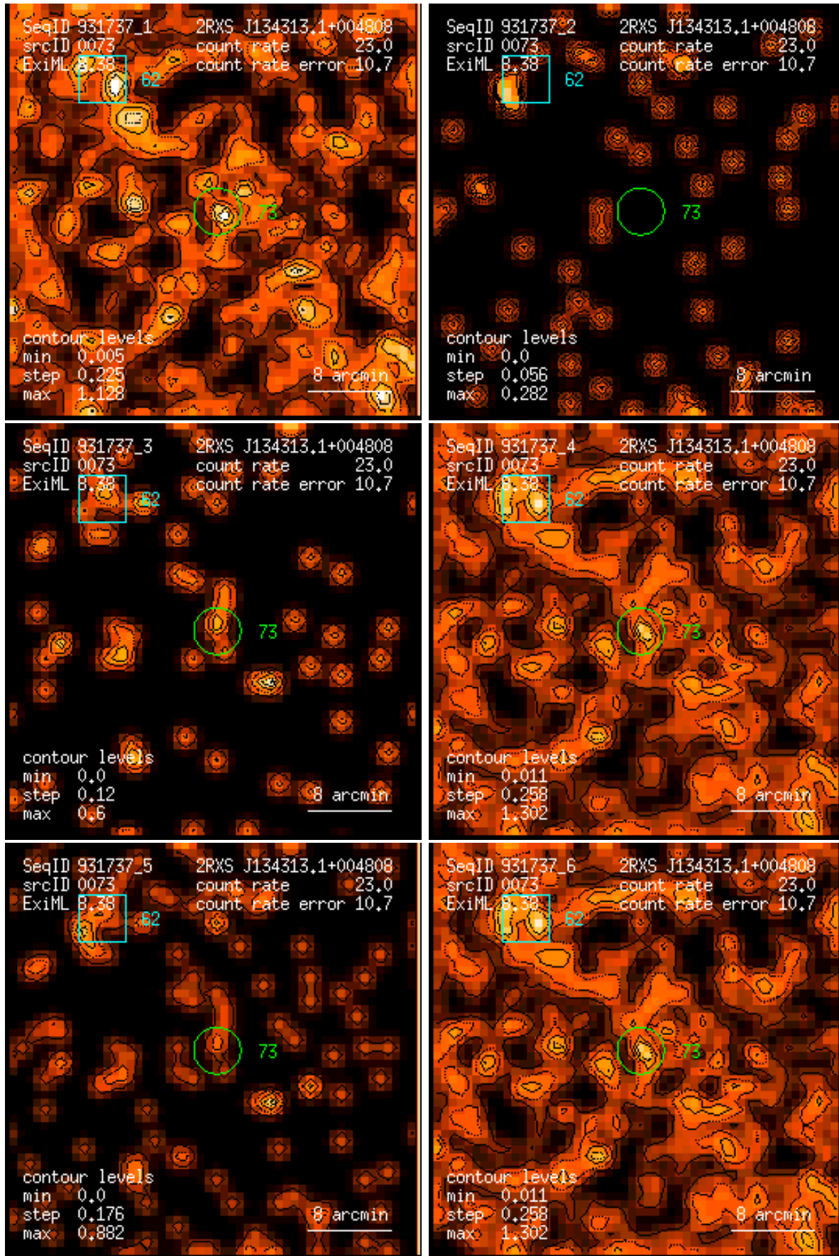
Figure 73: RASS 931737: detection 0073: band rate images, Gaussian filter: (1) PSPC channels 11 – 41, (2) 52 – 90, (3) 91 – 201, (4) 11 – 235, (5) 52 – 201, (6) 11 – 201. Broad band rates in counts/ks. Band rate contour levels in counts/ks/arcmin 2 .
