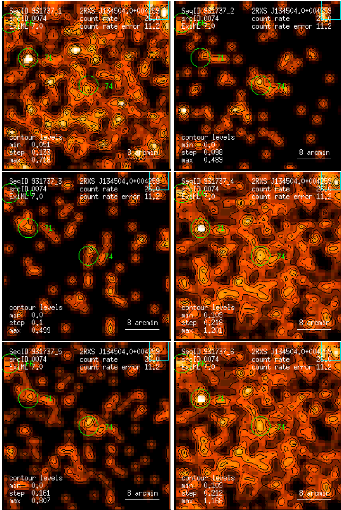
Figure 74: RASS 931737: detection 0074: band rate images, Gaussian filter: (1) PSPC channels 11 – 41, (2) 52 – 90, (3) 91 – 201, (4) 11 – 235, (5) 52 – 201, (6) 11 – 201. Broad band rates in counts/ks. Band rate contour levels in counts/ks/arcmin 2 .
