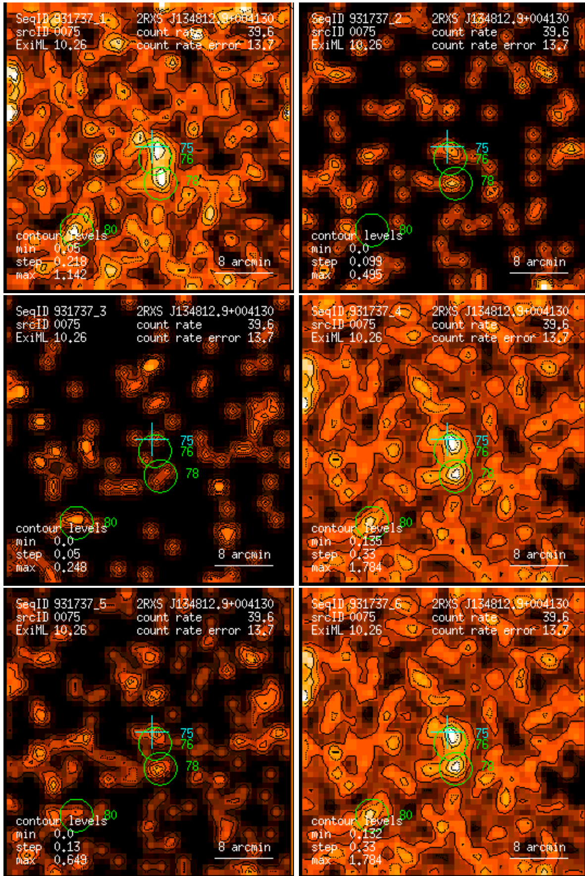
Figure 75: RASS 931737: detection 0075: band rate images, Gaussian filter: (1) PSPC channels 11 – 41, (2) 52 – 90, (3) 91 – 201, (4) 11 – 235, (5) 52 – 201, (6) 11 – 201. Broad band rates in counts/ks. Band rate contour levels in counts/ks/arcmin 2 .
