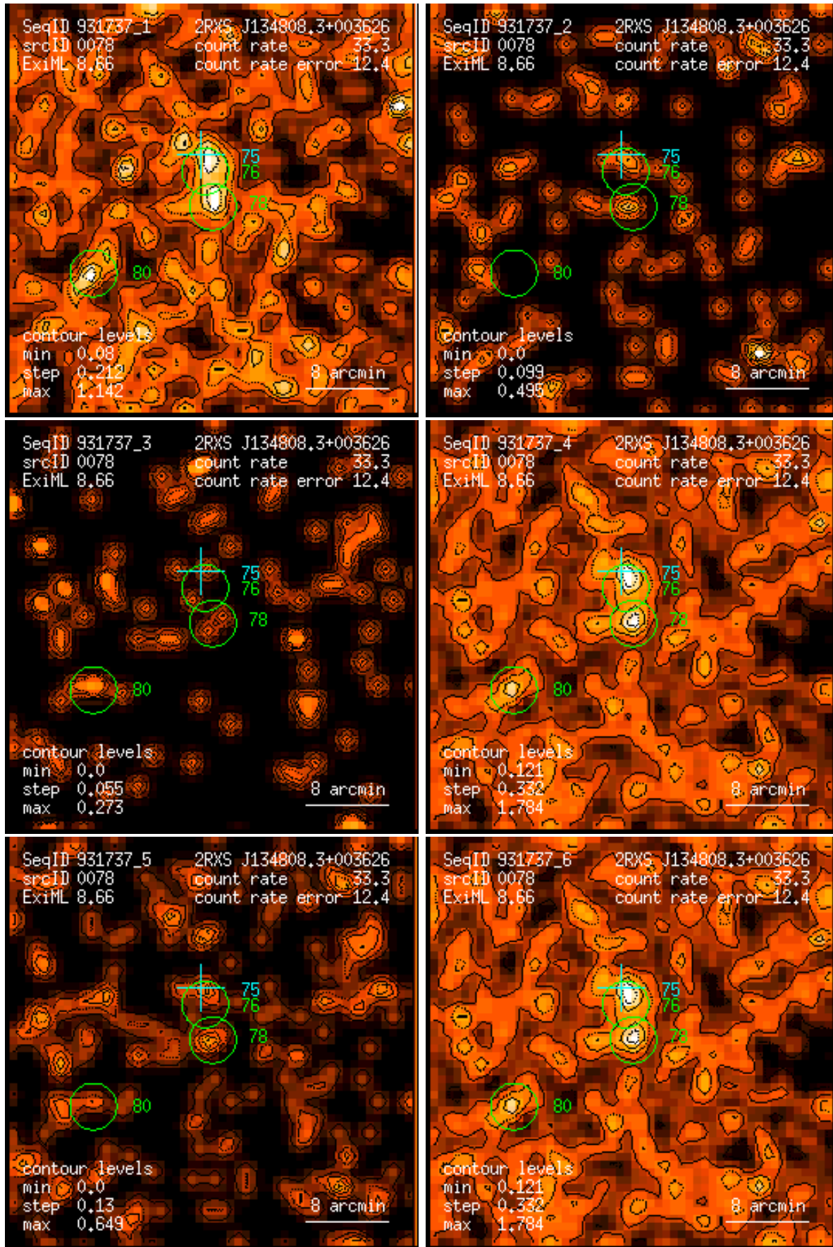
Figure 78: RASS 931737: detection 0078: band rate images, Gaussian filter: (1) PSPC channels 11 – 41, (2) 52 – 90, (3) 91 – 201, (4) 11 – 235, (5) 52 – 201, (6) 11 – 201. Broad band rates in counts/ks. Band rate contour levels in counts/ks/arcmin 2 .
