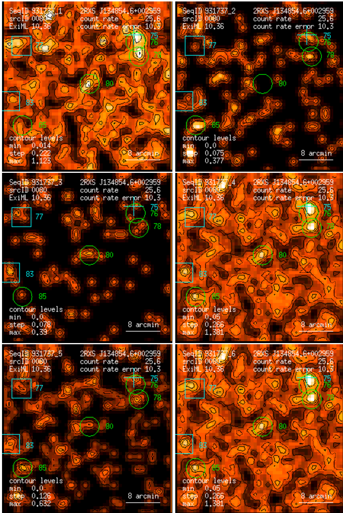
Figure 80: RASS 931737: detection 0080: band rate images, Gaussian filter: (1) PSPC channels 11 – 41, (2) 52 – 90, (3) 91 – 201, (4) 11 – 235, (5) 52 – 201, (6) 11 – 201. Broad band rates in counts/ks. Band rate contour levels in counts/ks/arcmin 2 .
