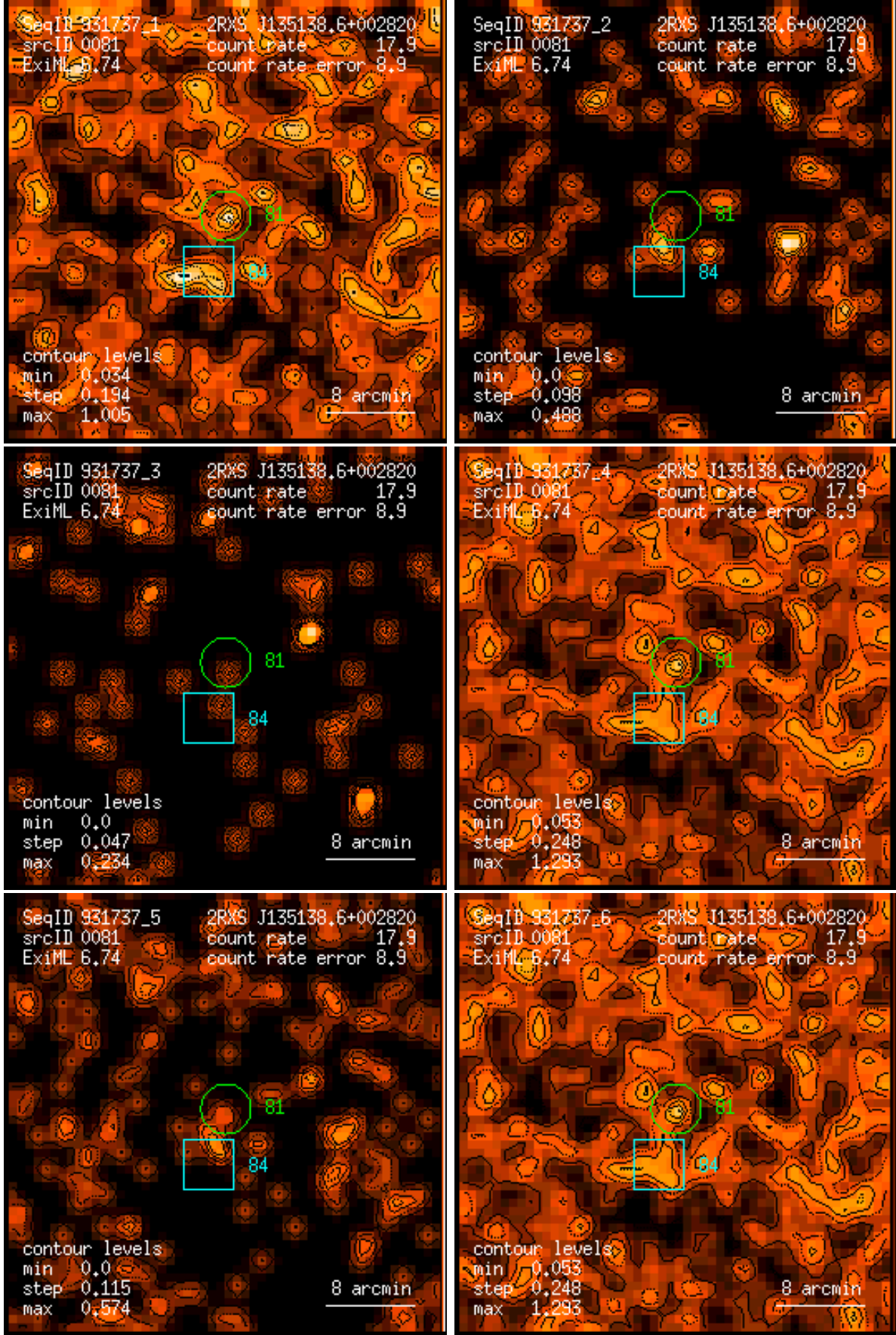
Figure 81: RASS 931737: detection 0081: band rate images, Gaussian filter: (1) PSPC channels 11 – 41, (2) 52 – 90, (3) 91 – 201, (4) 11 – 235, (5) 52 – 201, (6) 11 – 201. Broad band rates in counts/ks. Band rate contour levels in counts/ks/arcmin 2 .
