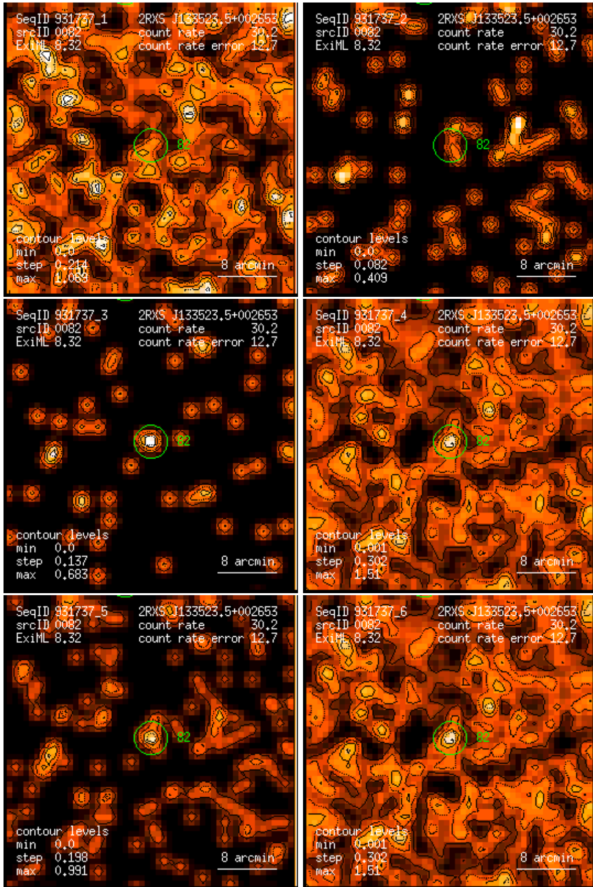
Figure 82: RASS 931737: detection 0082: band rate images, Gaussian filter: (1) PSPC channels 11 – 41, (2) 52 – 90, (3) 91 – 201, (4) 11 – 235, (5) 52 – 201, (6) 11 – 201. Broad band rates in counts/ks. Band rate contour levels in counts/ks/arcmin 2 .
